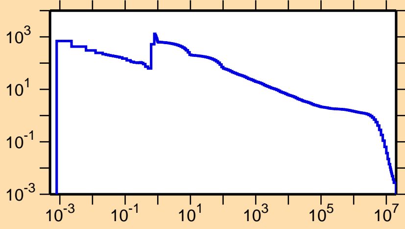
\sigma vs. E for ^{179}\text{Hg}(n,\gamma)
