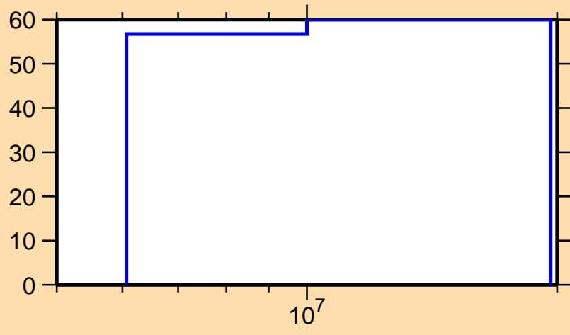
\Delta\sigma/\sigma vs. E for ^{179}\text{Hg}(n,\text{inel.})
