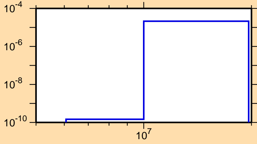
\sigma vs. E for ^{179}\text{Hg}(n,\text{pd})
