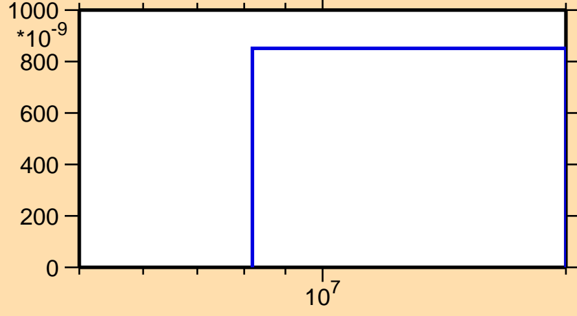
\sigma vs. E for ^{179}\text{Hg}(n,\text{pt})
