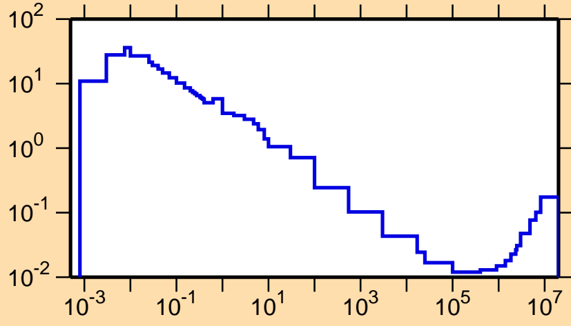
\sigma vs. E for ^{179}\text{Hg}(n,\alpha)
