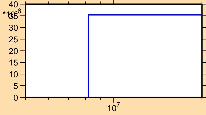
\sigma vs. E for ^{179}\text{Hg}(n,2np)
