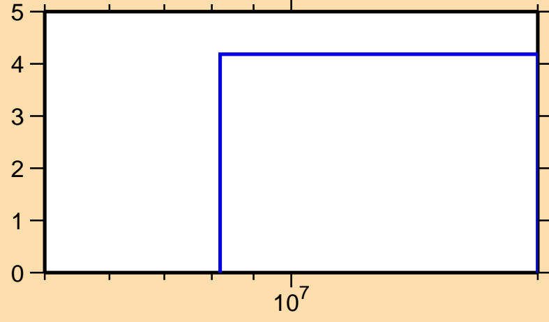
\Delta\sigma/\sigma vs. E for ^{179}\text{Hg}(n,\text{tot.})
