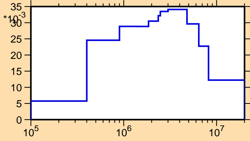
\sigma vs. E for ^{179}\text{Hg}(n,n_2)
