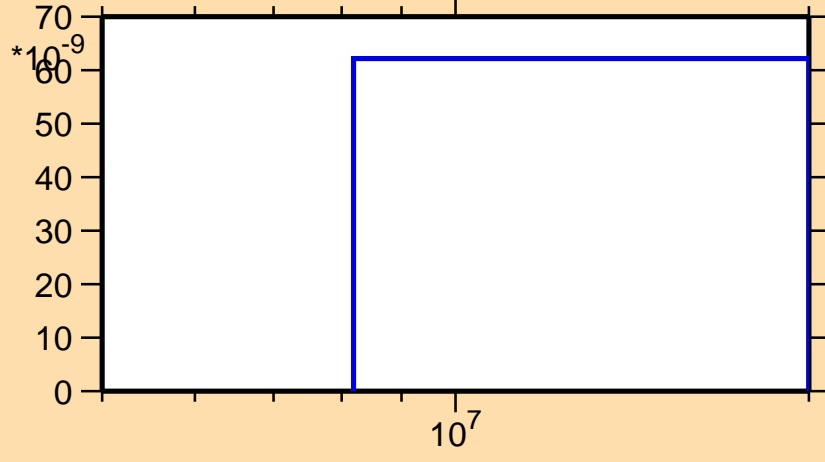
\sigma vs. E for ^{179}\text{Hg}(n,\text{nd})
