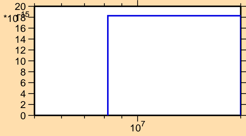
\sigma vs. E for ^{179}\text{Hg}(n,nt)
