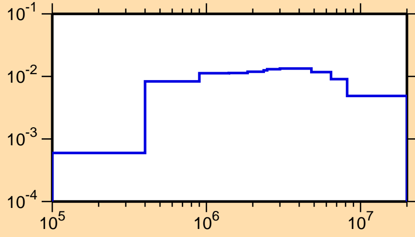
\sigma vs. E for ^{179}\text{Hg}(n,n_4)
