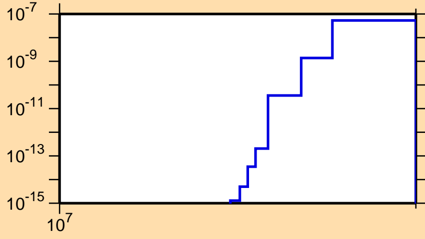
\sigma vs. E for ^{180}\text{Hg}(n,\text{nd})
