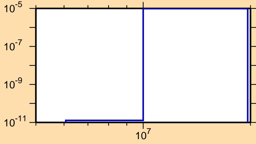
\sigma vs. E for ^{180}\text{Hg}(n,\text{pd})
