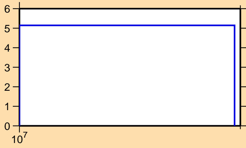
\Delta\sigma/\sigma vs. E for ^{180}\text{Hg}(n,\text{tot.})
