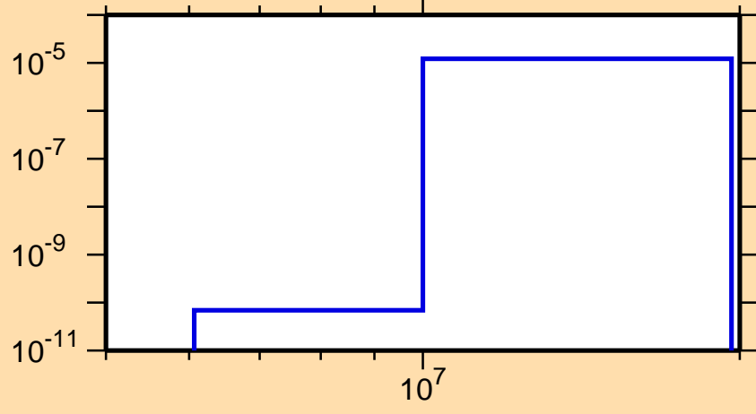
\sigma vs. E for ^{180}\text{Hg}(\text{mt } 45)
