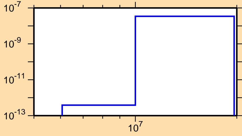
\sigma vs. E for ^{180}\text{Hg}(\text{mt117})
