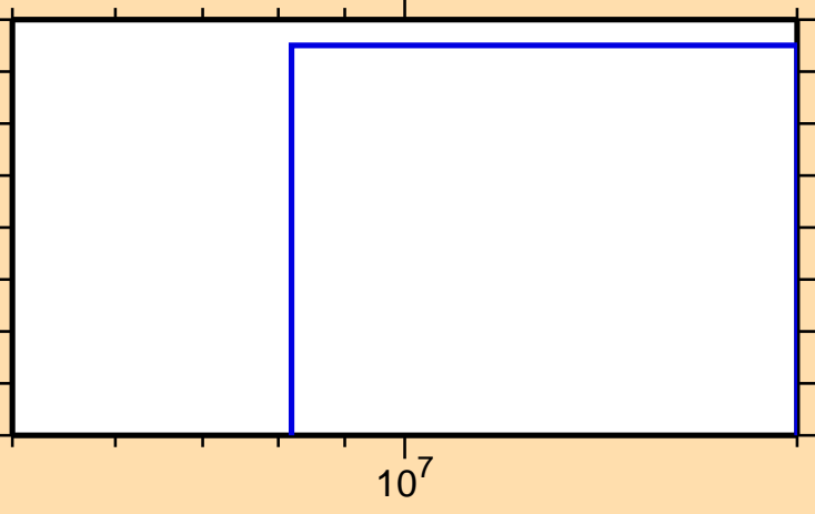
\sigma vs. E for ^{180}\text{Hg}(n,2n)
