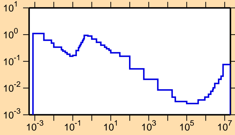
\sigma vs. E for ^{180}\text{Hg}(n,\alpha)
