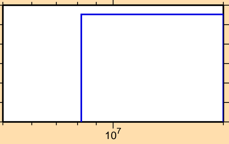
\sigma vs. E for ^{180}\text{Hg}(\text{mt117})
