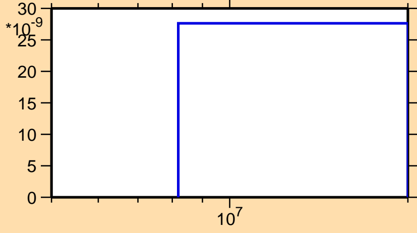
\sigma vs. E for ^{180}\text{Hg}(\text{mt117})
