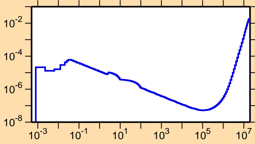
\sigma vs. E for ^{181}\text{Hg}(n,p\alpha)
