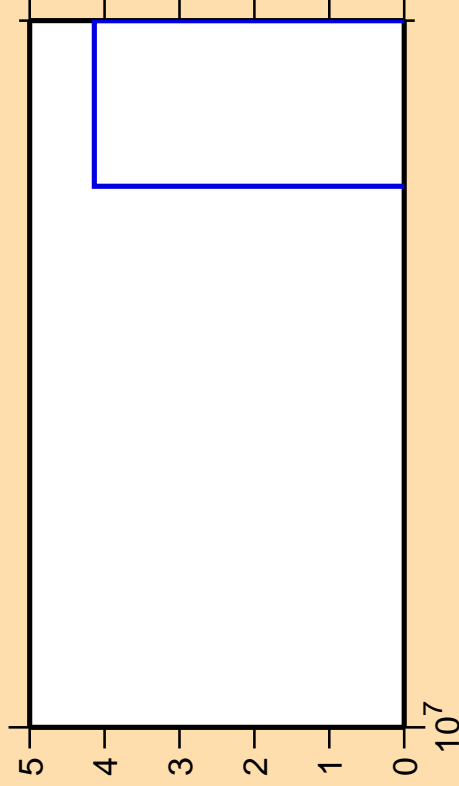
\Delta\sigma/\sigma vs. E for ^{181}\text{Hg}(n,3n)
