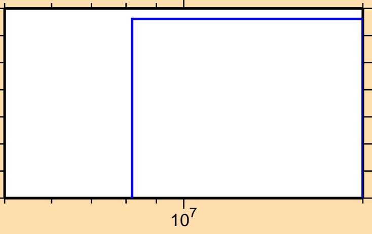
\sigma vs. E for ^{181}\text{Hg}(n,2np)
