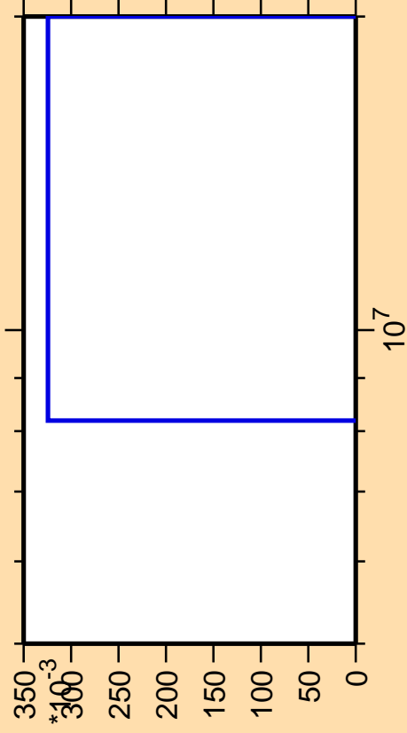
\Delta\sigma/\sigma vs. E for ^{181}\text{Hg}(n,nt)
