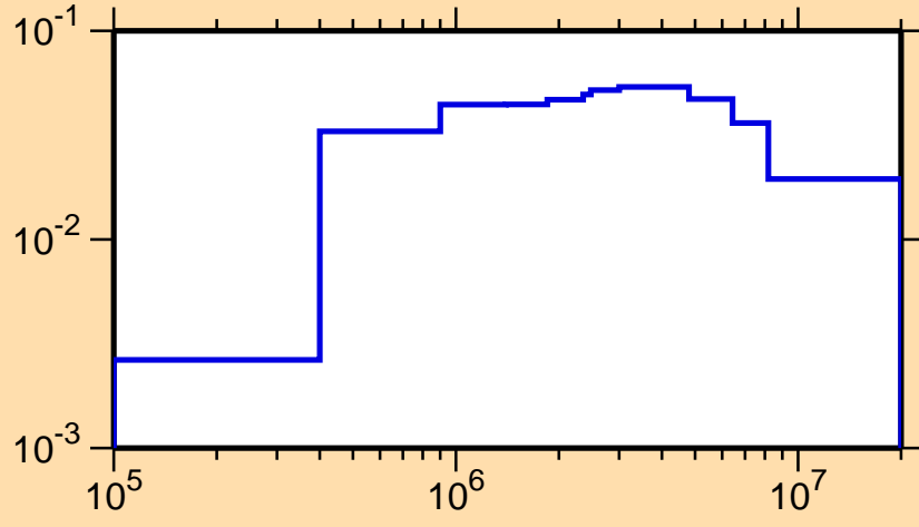
\sigma vs. E for ^{181}\text{Hg}(n,n_4)
