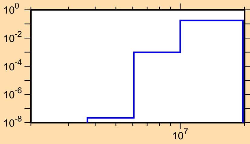
\sigma vs. E for ^{182}\text{Hg}(n,np)
