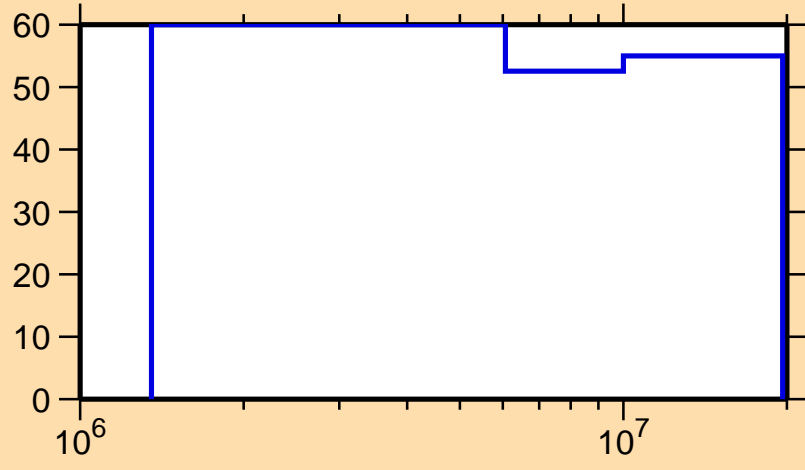
\Delta\sigma/\sigma vs. E for ^{182}\text{Hg}(n,n\text{cont.})
