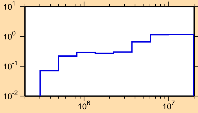
\sigma vs. E for ^{182}\text{Hg}(n,\text{inel.})
