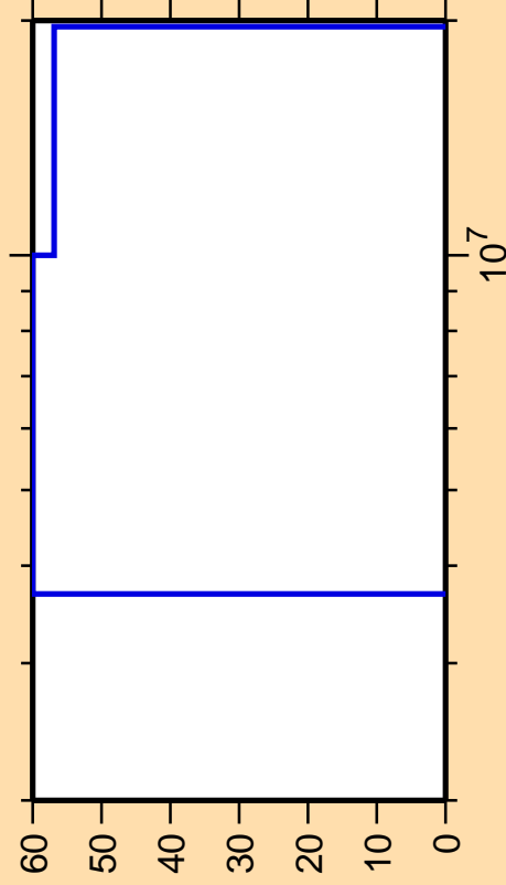
\Delta\sigma/\sigma vs. E for ^{182}\text{Hg}(n,np)
