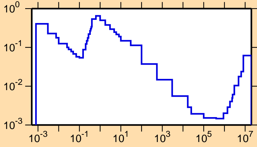
\sigma vs. E for ^{182}\text{Hg}(n,\alpha)
