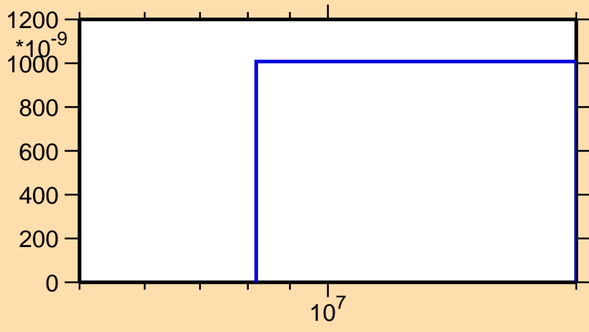
\sigma vs. E for ^{182}\text{Hg}(n,\text{pd})
