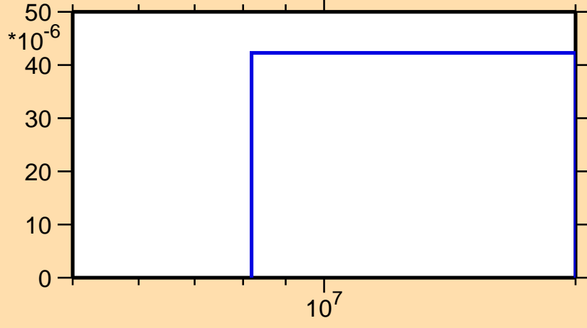
\sigma vs. E for ^{182}\text{Hg}(n,t)
