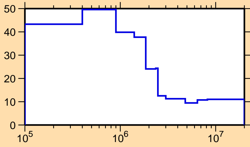
\Delta\sigma/\sigma vs. E for ^{182}\text{Hg}(n,\text{nonel.})
