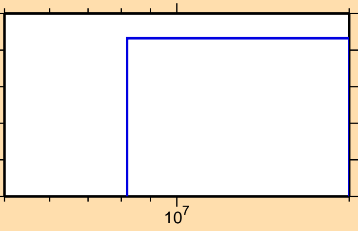
\sigma vs. E for ^{182}\text{Hg}(n,\text{nd})
