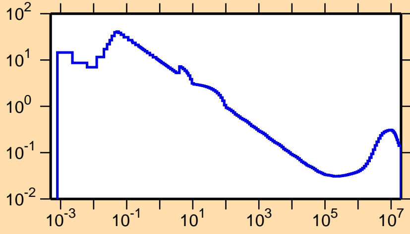
\sigma vs. E for ^{183}\text{Hg}(n,p)
