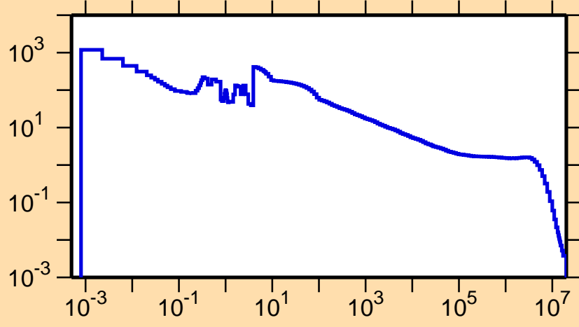
\sigma vs. E for ^{183}\text{Hg}(n,\gamma)
