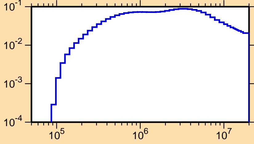
\sigma vs. E for ^{183}\text{Hg}(n,n_2)
