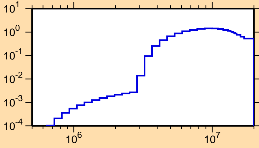
\sigma vs. E for ^{183}\text{Hg}(n,n\text{cont.})
