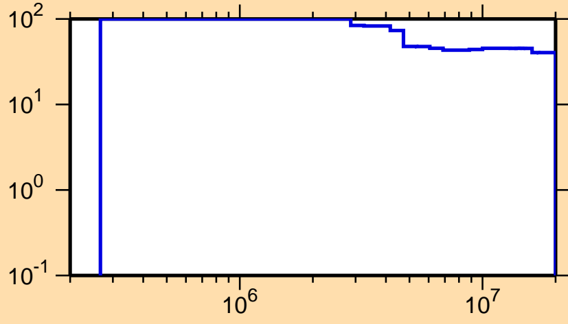
\Delta\sigma/\sigma vs. E for ^{183}\text{Hg}(n,n\text{cont.})
