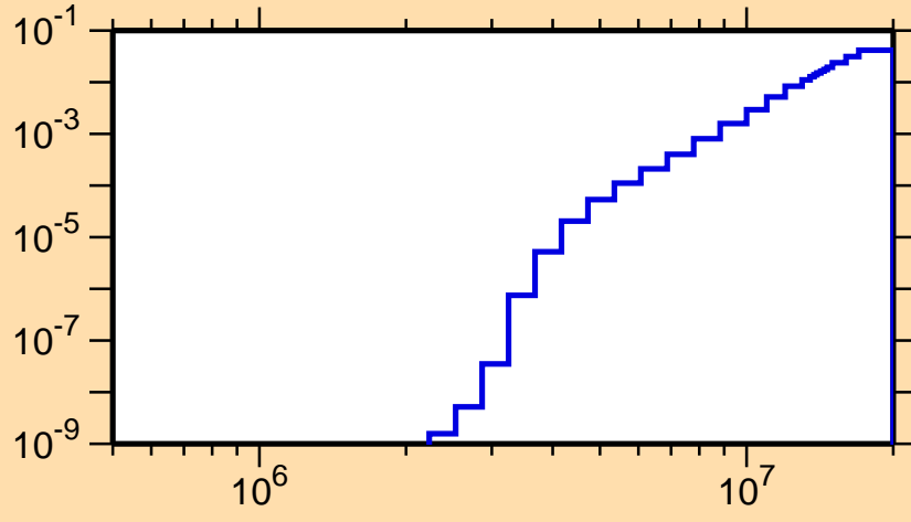
\sigma vs. E for ^{183}\text{Hg}(n,n\alpha)
