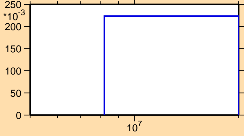
\sigma vs. E for ^{183}\text{Hg}(n,2n)
