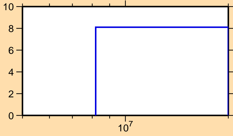
\Delta\sigma/\sigma vs. E for ^{183}\text{Hg}(n,\text{nonel.})
