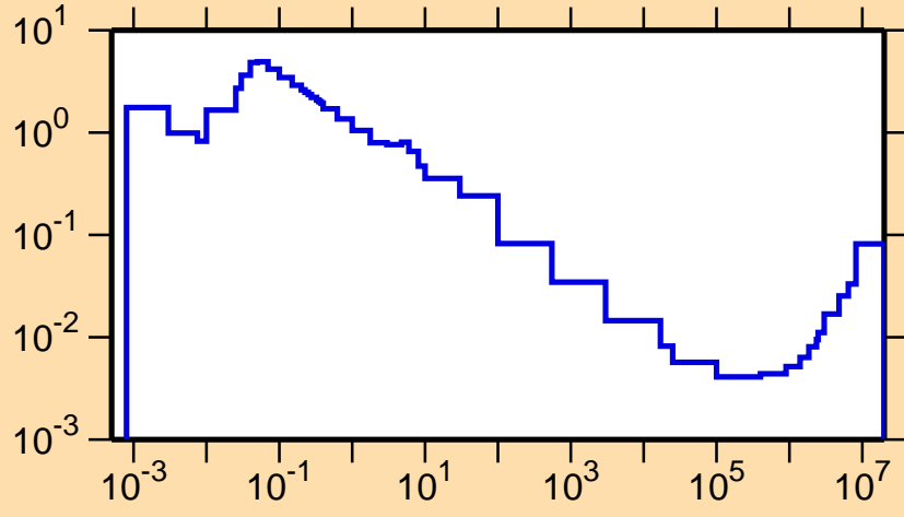
\sigma vs. E for ^{183}\text{Hg}(n,\alpha)
