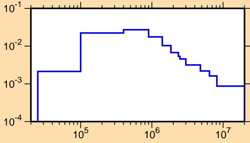
\sigma vs. E for ^{183}\text{Hg}(n,n_1)
