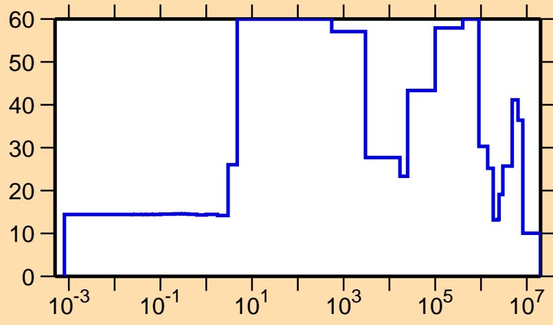
\Delta\sigma/\sigma vs. E for ^{183}\text{Hg}(n,\text{el.})
