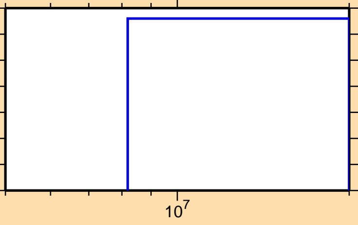
\sigma vs. E for ^{183}\text{Hg}(n,2n\alpha)
