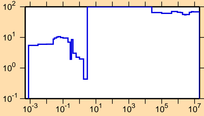
\Delta\sigma/\sigma vs. E for ^{183}\text{Hg}(n,\gamma)
