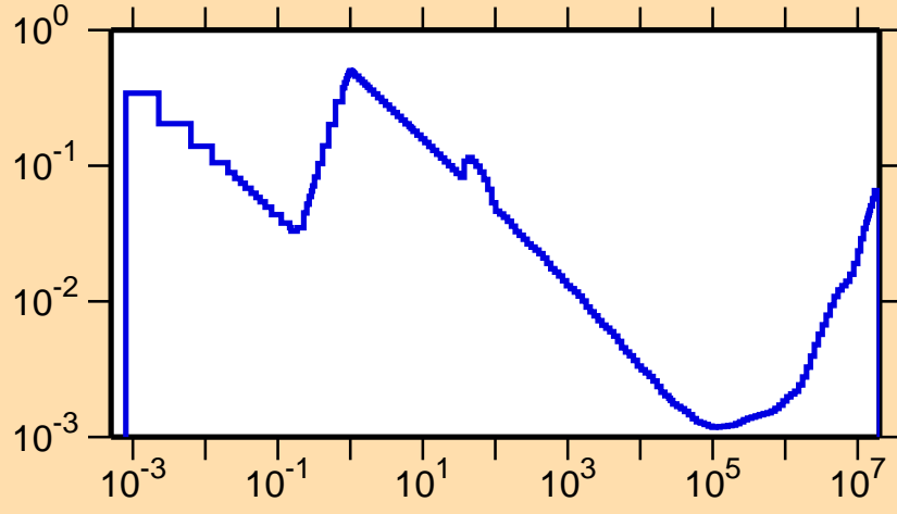
\sigma vs. E for ^{184}\text{Hg}(n,\alpha)
