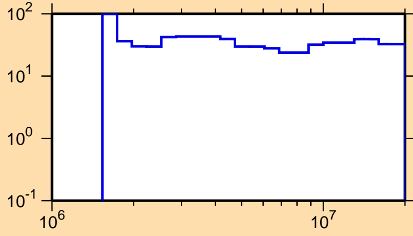
\Delta\sigma/\sigma vs. E for ^{184}\text{Hg}(n,n\text{cont.})
