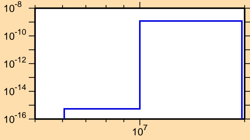
\sigma vs. E for ^{184}\text{Hg}(\text{mt117})
