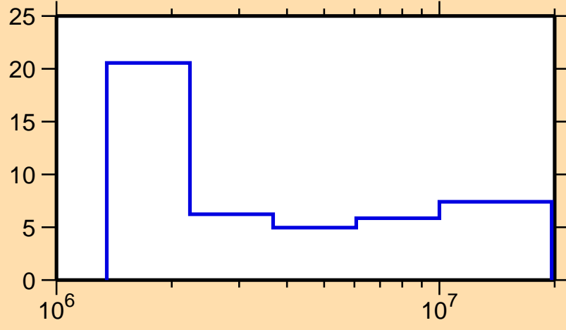
\Delta\sigma/\sigma vs. E for ^{184}\text{Hg}(n,n\text{onel.})
