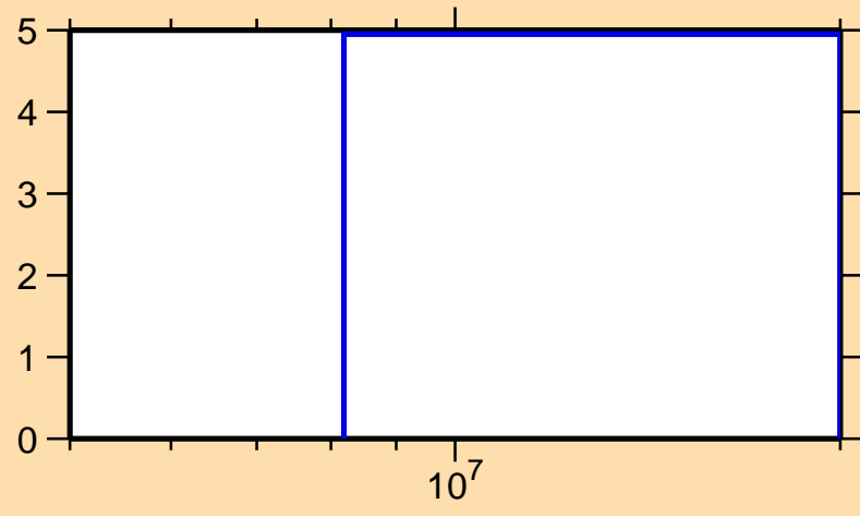
\Delta\sigma/\sigma vs. E for ^{184}\text{Hg}(n,\text{el.})
