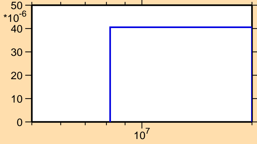
\sigma vs. E for ^{184}\text{Hg}(n,t)
