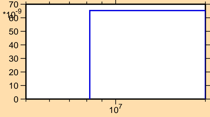
\sigma vs. E for ^{184}\text{Hg}(n,\text{pd})
