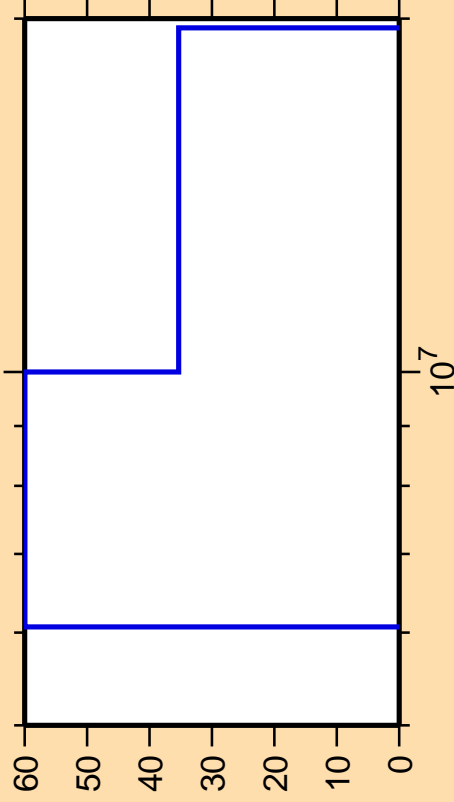
\Delta\sigma/\sigma vs. E for ^{185}\text{Hg}(n,2n)
