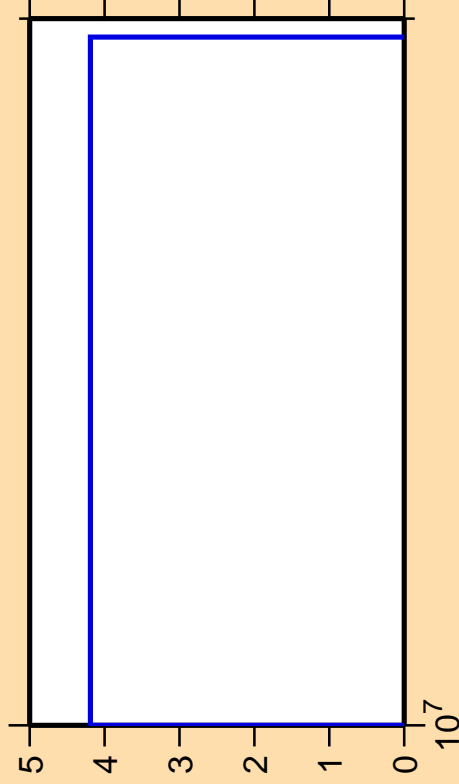
\Delta\sigma/\sigma vs. E for ^{185}\text{Hg}(n,nt)
