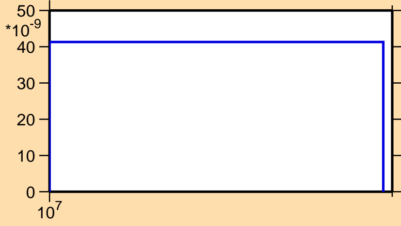
\sigma vs. E for ^{185}\text{Hg}(n,\text{nd})
