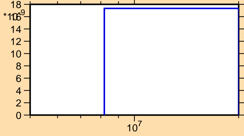
\sigma vs. E for ^{185}\text{Hg}(n,\text{pd})
