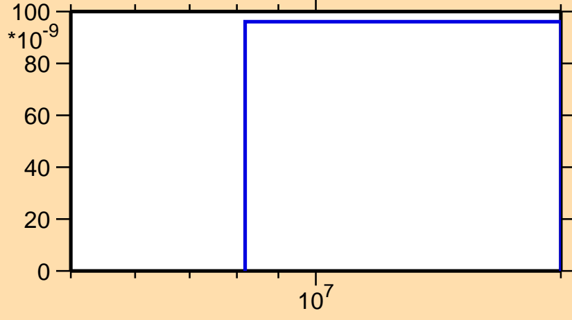
\sigma vs. E for ^{185}\text{Hg} (mt 45)
