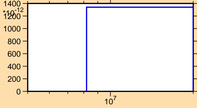
\sigma vs. E for ^{185}\text{Hg}(n,\text{pt})
