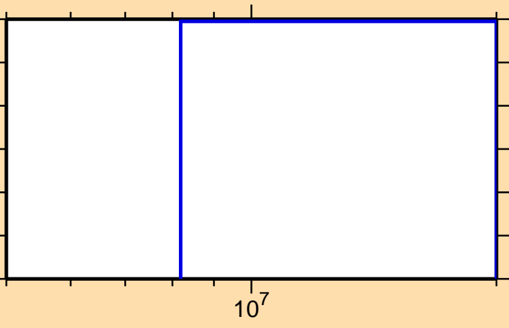
\sigma vs. E for ^{185}\text{Hg}(n,2np)
