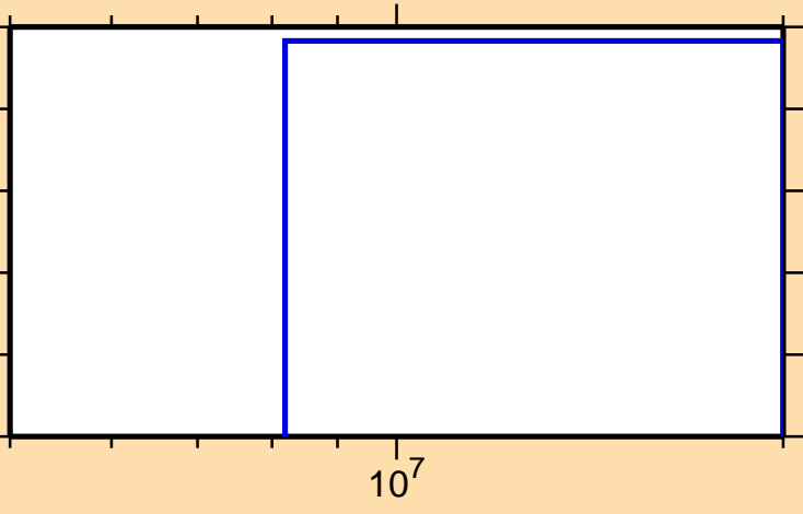
\sigma vs. E for ^{185}\text{Hg}(n,2n\alpha)
