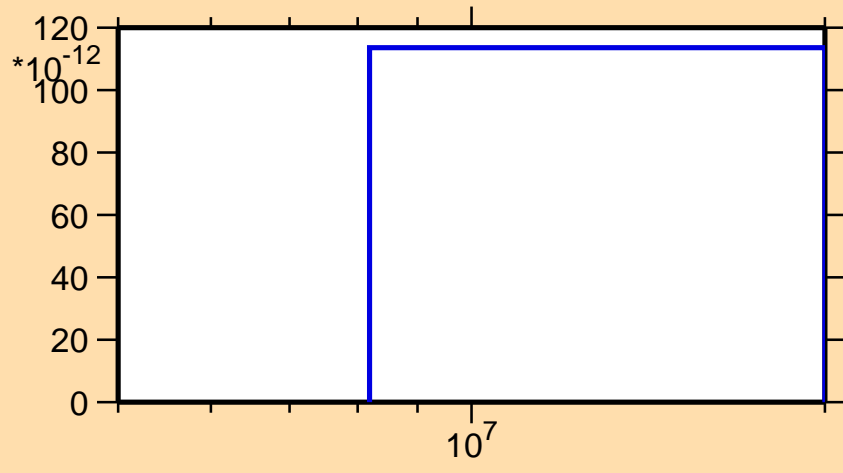
\sigma vs. E for ^{185}\text{Hg}(n,3n\alpha)
