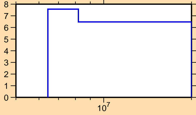
\Delta\sigma/\sigma vs. E for ^{185}\text{Hg}(n,\text{nonel.})
