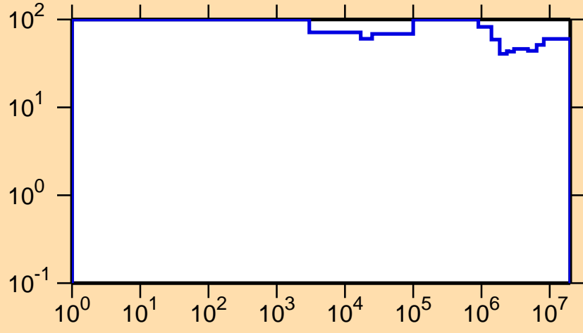
\Delta\sigma/\sigma vs. E for ^{185}\text{Hg}(n,n_1)
