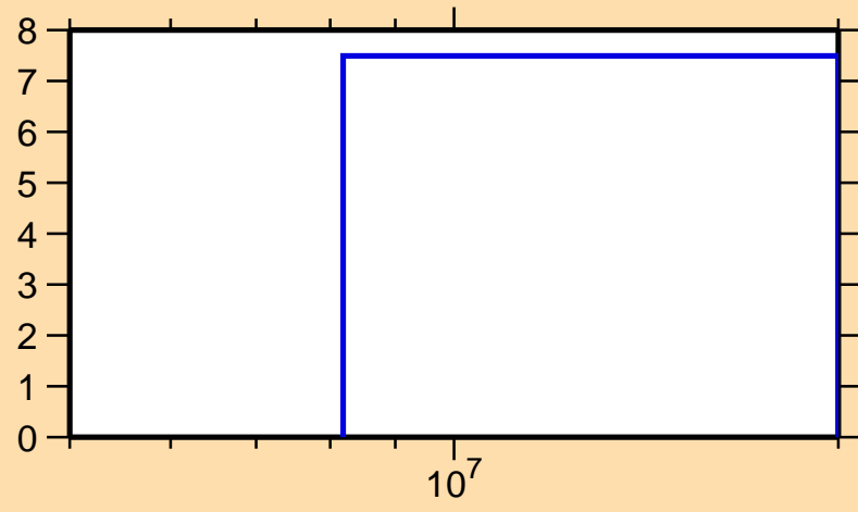
\Delta\sigma/\sigma vs. E for ^{186}\text{Hg}(n,\text{nonel.})
