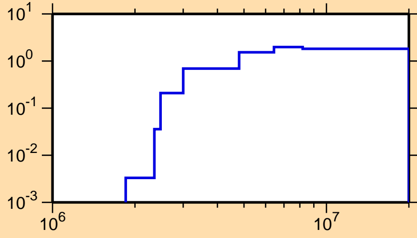
\sigma vs. E for ^{186}\text{Hg}(n,n\text{cont.})
