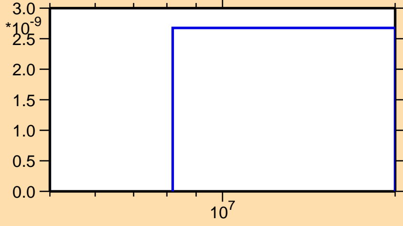
\sigma vs. E for ^{186}\text{Hg}(n,\text{pd})
