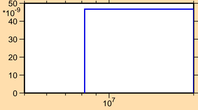
\sigma vs. E for ^{186}\text{Hg}(n,2np)
