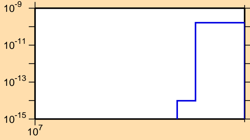
\sigma vs. E for ^{187}\text{Hg}(n,nt)
