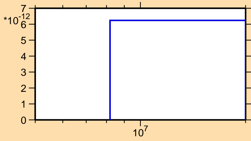
\sigma vs. E for ^{187}\text{Hg} (mt 34)
