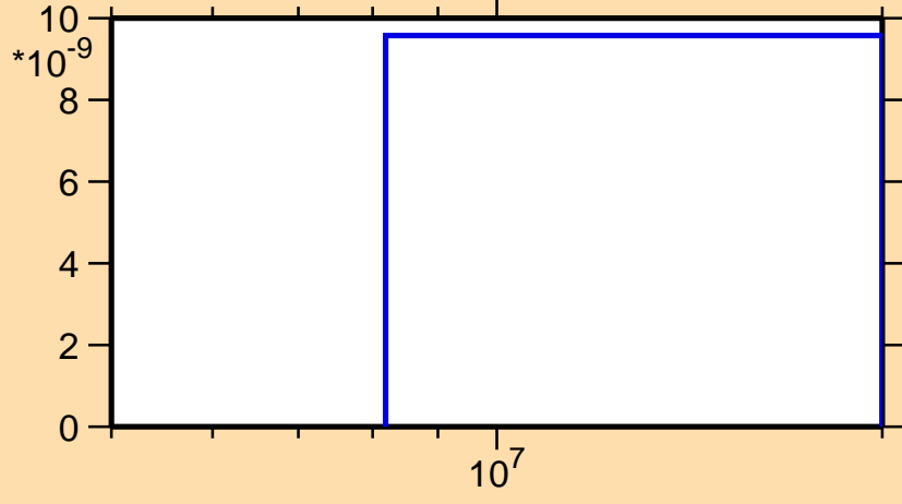
\sigma vs. E for ^{187}\text{Hg} (mt 45)
