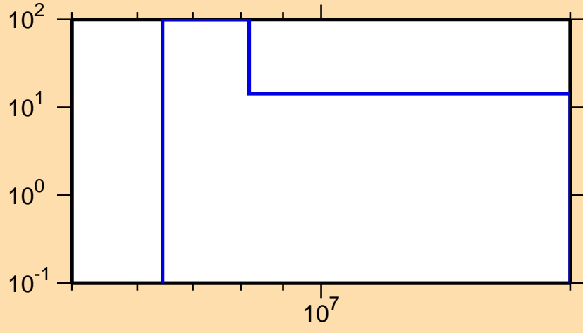
\Delta\sigma/\sigma vs. E for ^{187}\text{Hg}(n,2n)
