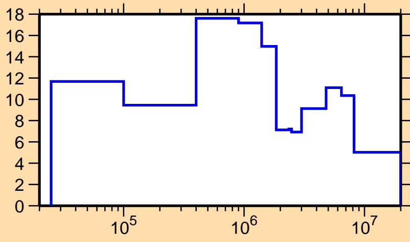
\Delta\sigma/\sigma vs. E for ^{187}\text{Hg}(n,\text{tot.})
