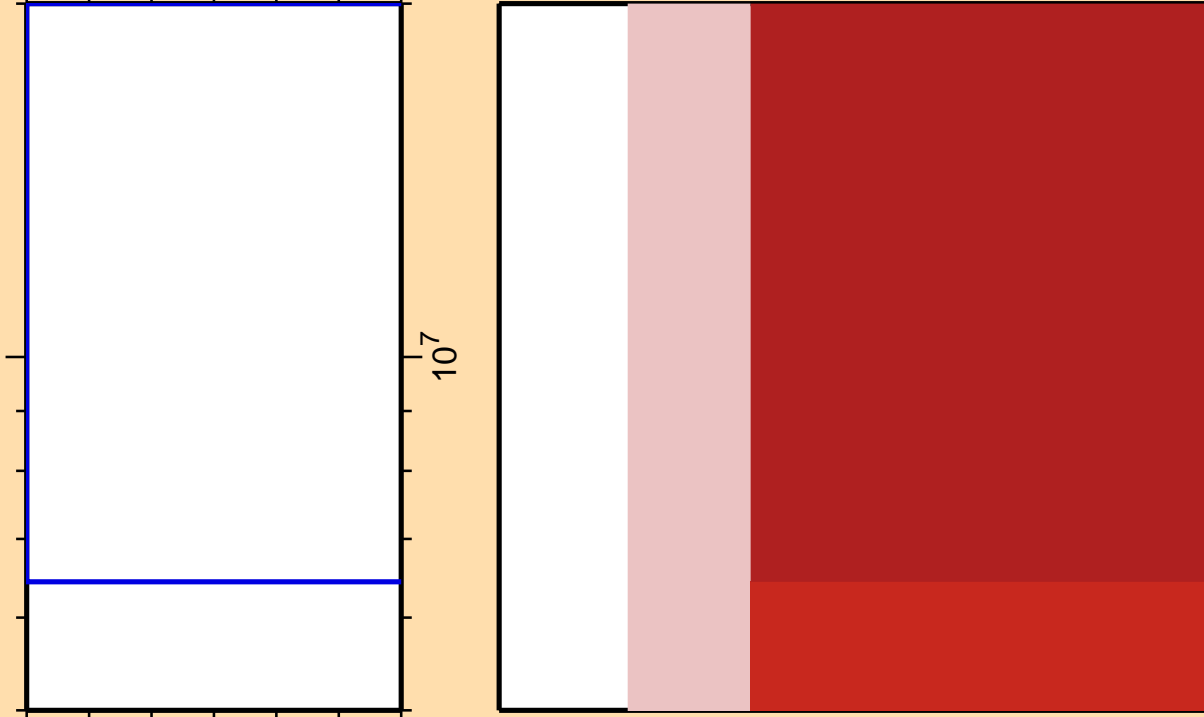
\Delta\sigma/\sigma vs. E for ^{187}\text{Hg}(n,\gamma)
