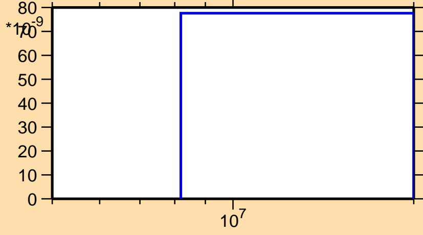
\sigma vs. E for ^{187}\text{Hg}(n,\text{nd})
