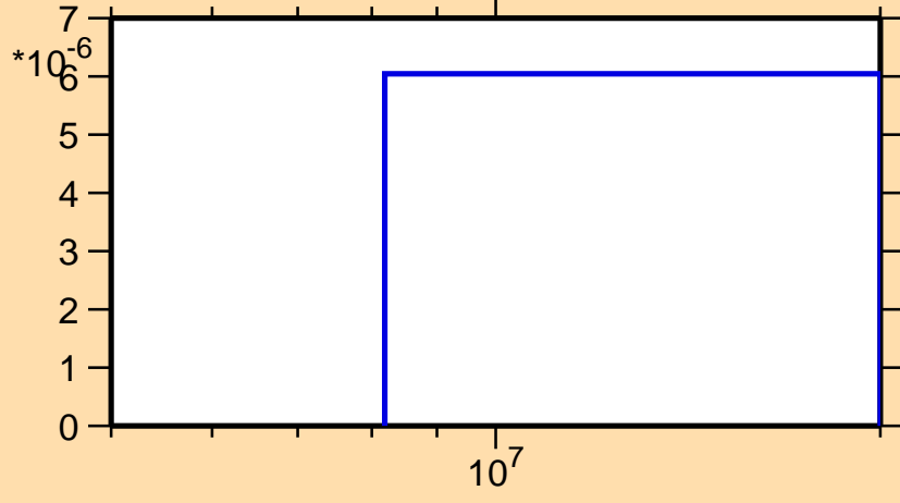
\sigma vs. E for ^{187}\text{Hg}(n,2np)
