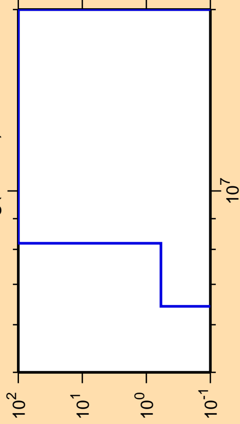
\Delta\sigma/\sigma vs. E for ^{187}\text{Hg}(n,\text{He}3)
