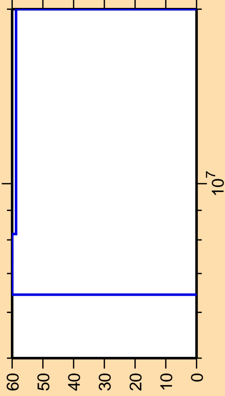
\Delta\sigma/\sigma vs. E for ^{187}\text{Hg}(n,n_1)
