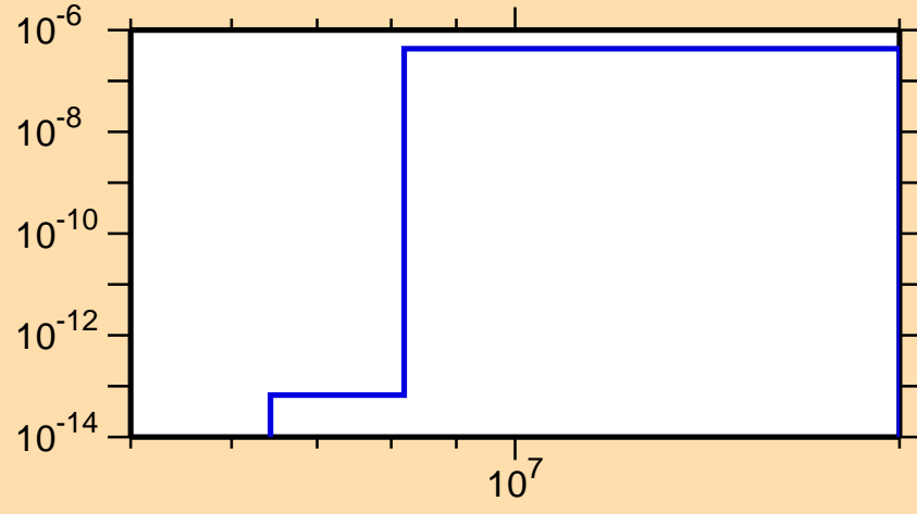
\sigma vs. E for ^{187}\text{Hg}(n,\text{He}3)
