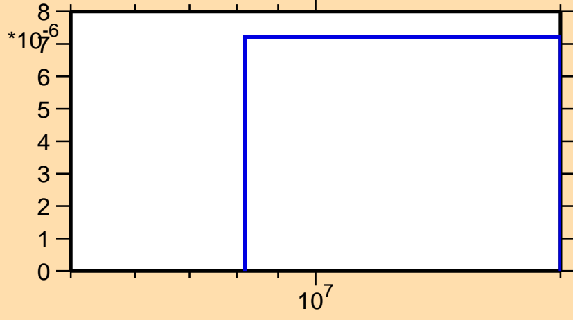
\sigma vs. E for ^{187}\text{Hg}(n,2n\alpha)
