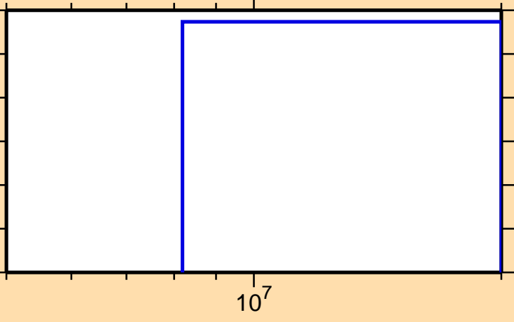
\sigma vs. E for ^{187}\text{Hg}(n,3n)
