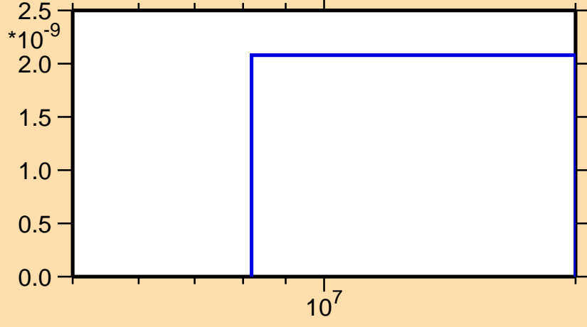
\sigma vs. E for ^{187}\text{Hg}(n,\text{pd})
