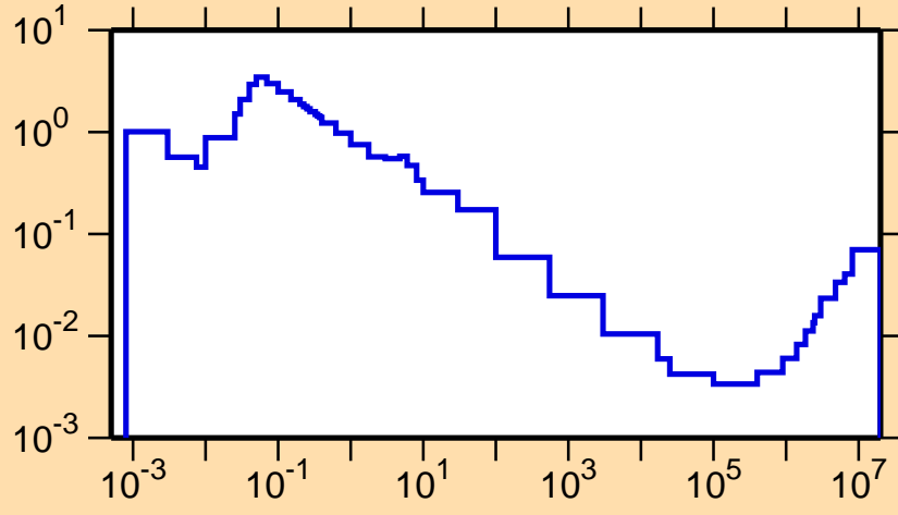
\sigma vs. E for ^{187}\text{Hg}(n,p)
