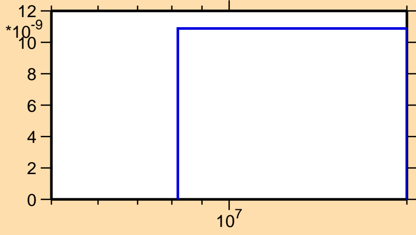
\sigma vs. E for ^{187}\text{Hg} (mt 45)
