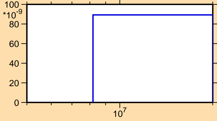
\sigma vs. E for ^{187}\text{Hg}(n,\text{nd})
