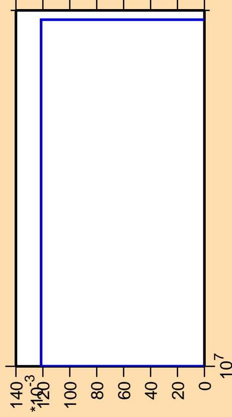
\Delta\sigma/\sigma vs. E for ^{188}\text{Hg}(n,3n\alpha)
