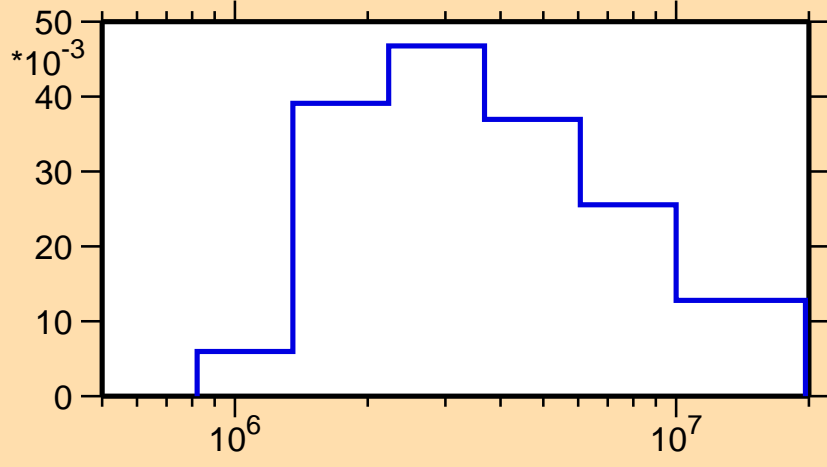
\sigma vs. E for ^{188}\text{Hg}(n,n_4)
