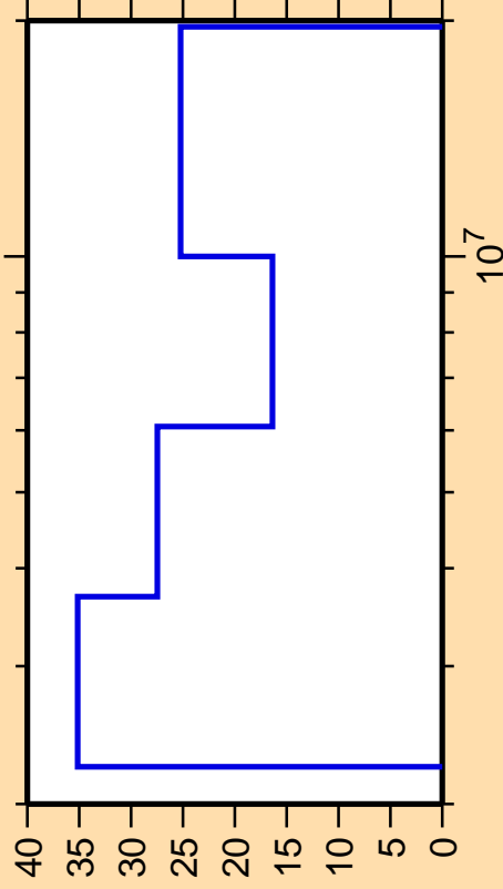
\Delta\sigma/\sigma vs. E for ^{188}\text{Hg}(n,n\text{cont.})
