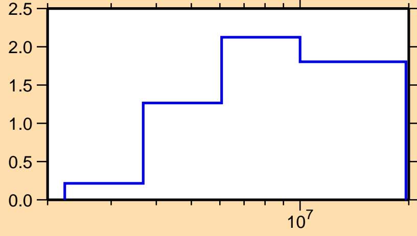
\sigma vs. E for ^{188}\text{Hg}(n,n\text{cont.})
