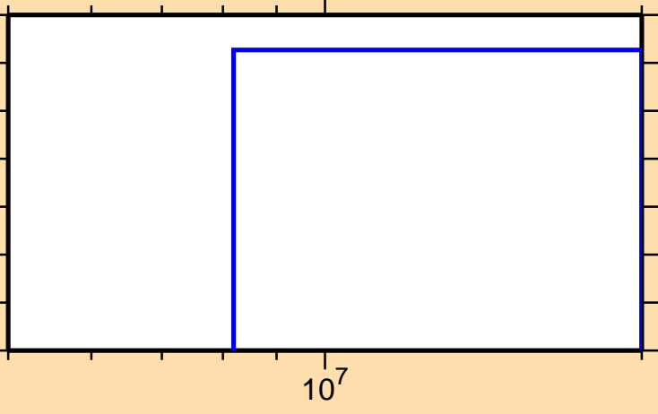
\sigma vs. E for ^{188}\text{Hg}(n,2np)
