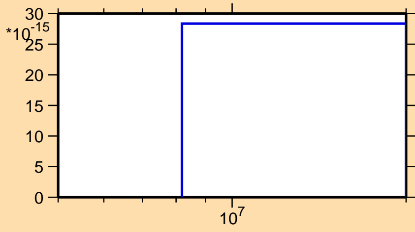
\sigma vs. E for ^{188}\text{Hg}(n,3n\alpha)
