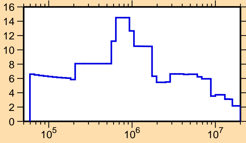
\Delta\sigma/\sigma vs. E for ^{189}\text{Hg}(n,\text{tot.})
