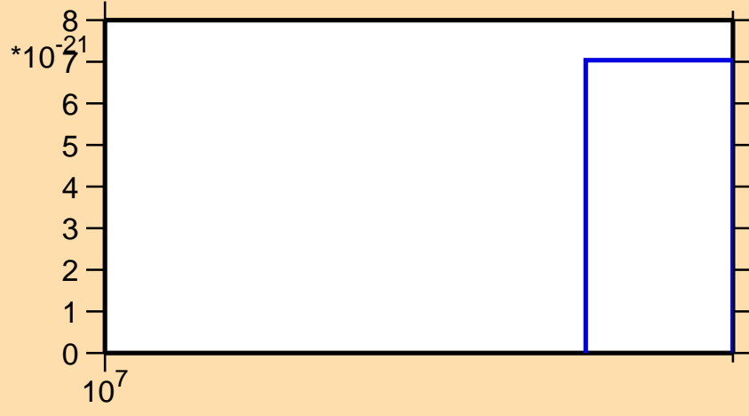
\sigma vs. E for ^{189}\text{Hg} (mt 11)
