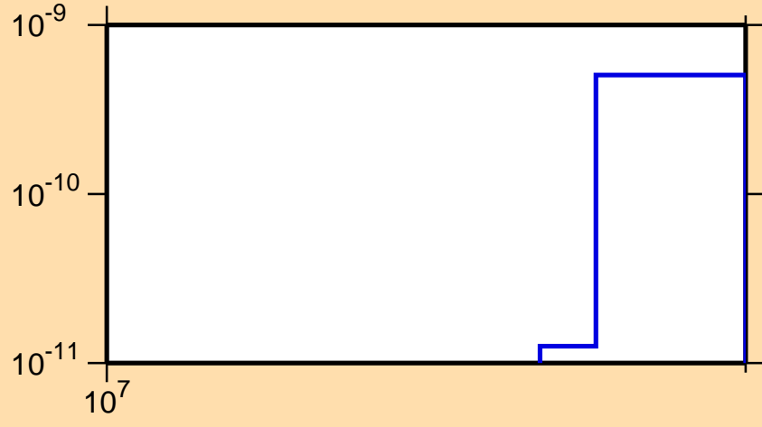
\sigma vs. E for ^{189}\text{Hg}(n,\text{pt})
