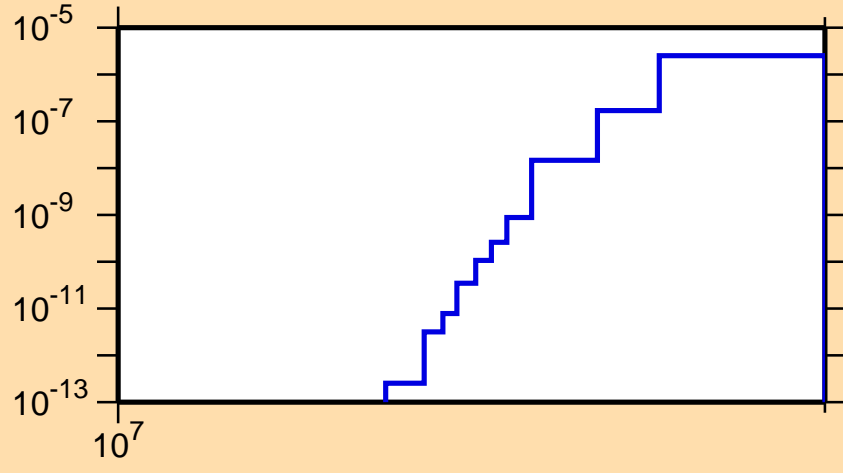
\sigma vs. E for ^{189}\text{Hg}(n,\text{nd})
