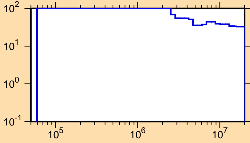
\Delta\sigma/\sigma vs. E for ^{189}\text{Hg}(n,n_1)
