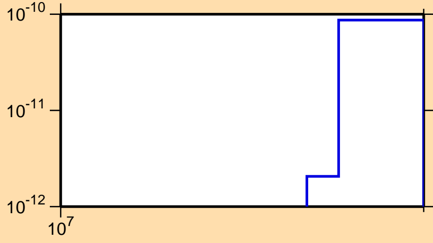
\sigma vs. E for ^{189}\text{Hg} (mt 34)
