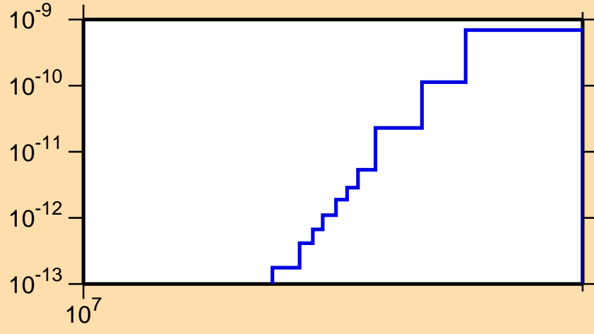
\sigma vs. E for ^{189}\text{Hg}(\text{mt117})
