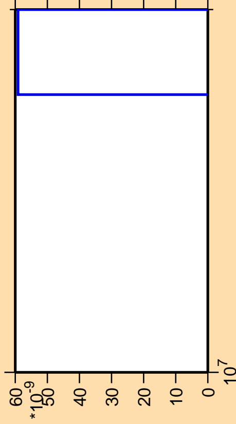
\Delta\sigma/\sigma vs. E for ^{189}\text{Hg} (mt 11)
