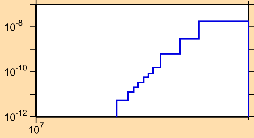
\sigma vs. E for ^{189}\text{Hg} (mt 45)
