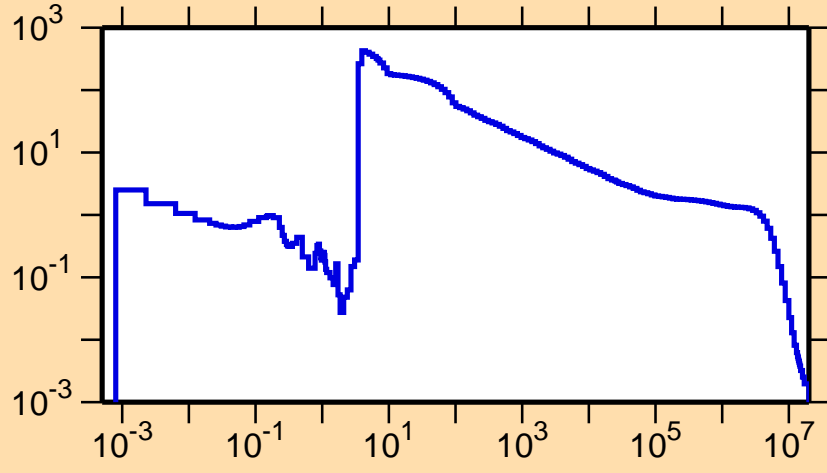
\sigma vs. E for ^{189}\text{Hg}(n,\gamma)
