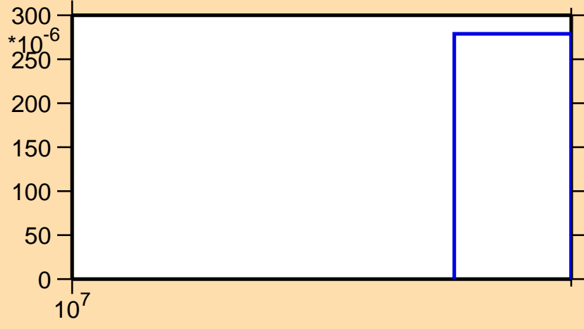
\sigma vs. E for ^{189}\text{Hg}(n,3n)
