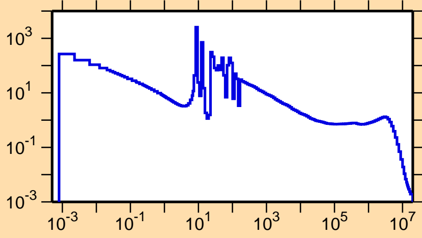
\sigma vs. E for ^{190}\text{Hg}(n,\gamma)
