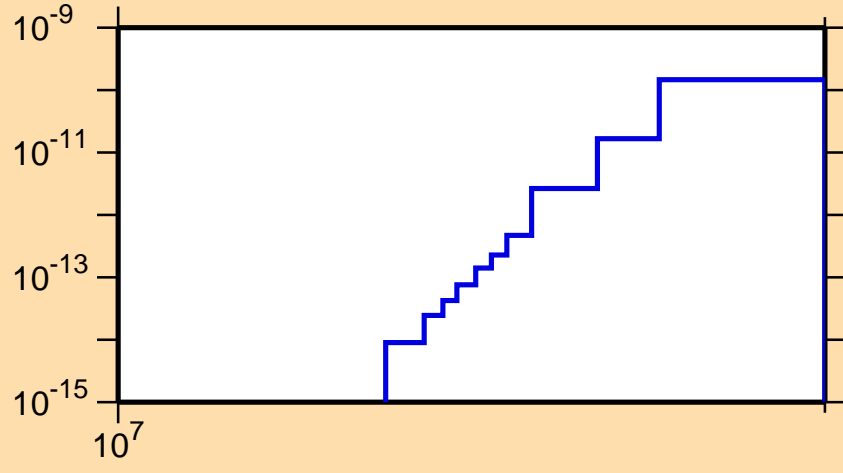
\sigma vs. E for ^{190}\text{Hg}(\text{mt117})
