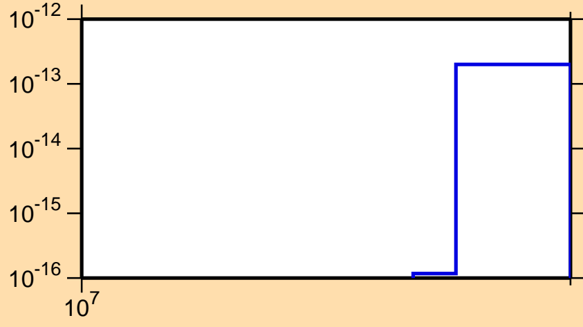
\sigma vs. E for ^{190}\text{Hg}(n,\text{pt})
