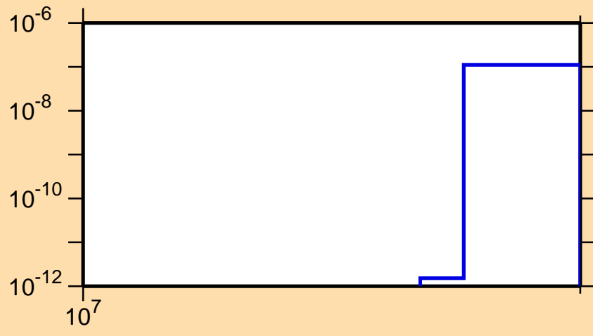
\sigma vs. E for ^{190}\text{Hg}(n,2np)
