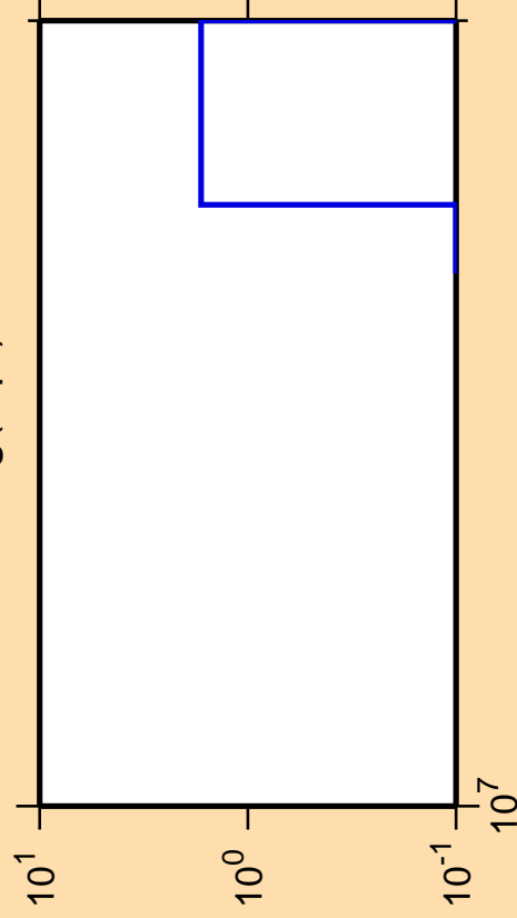
\Delta\sigma/\sigma vs. E for ^{190}\text{Hg}(n,\text{pt})
