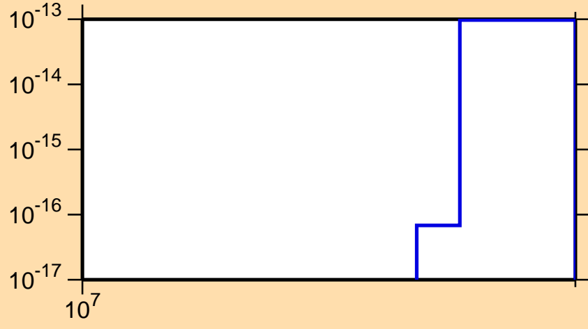
\sigma vs. E for ^{190}\text{Hg} (mt 34)
