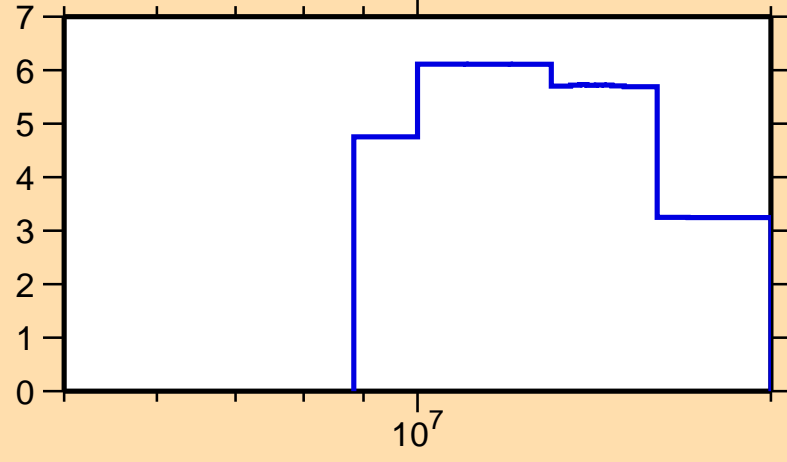
\Delta\sigma/\sigma vs. E for ^{190}\text{Hg}(n,\text{el.})
