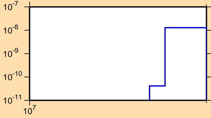
\sigma vs. E for ^{190}\text{Hg}(n,\text{nd})
