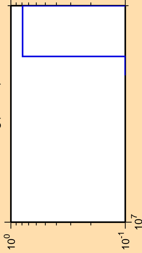
\Delta\sigma/\sigma vs. E for ^{190}\text{Hg} (mt 34)
