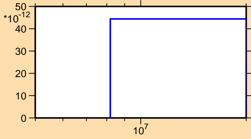
\sigma vs. E for ^{190}\text{Hg}(\text{mt } 45)
