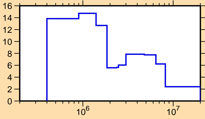
\Delta\sigma/\sigma vs. E for ^{190}\text{Hg}(n,\text{tot.})
