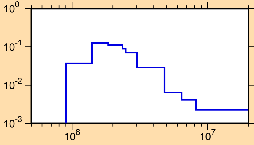
\sigma vs. E for ^{190}\text{Hg}(n,n_3)
