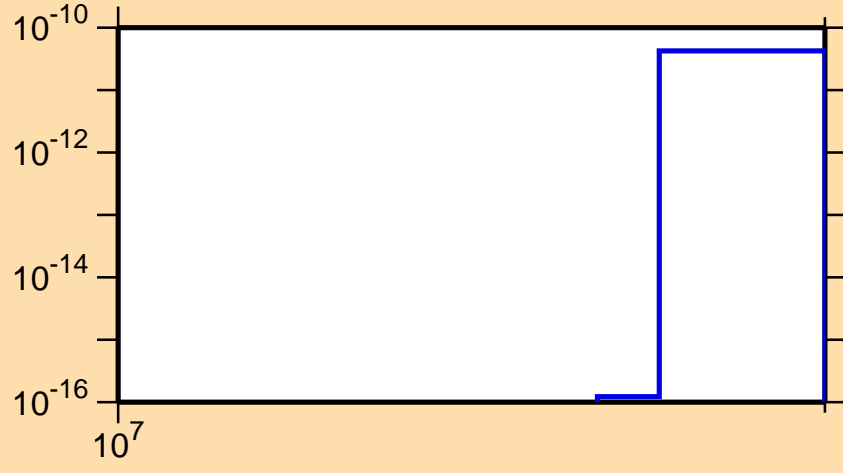
\sigma vs. E for ^{191}\text{Hg}(n,nt)
