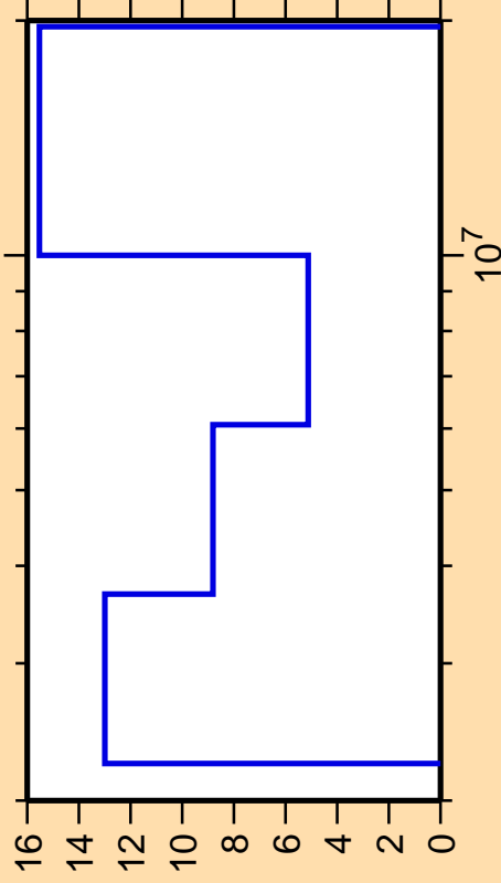
\Delta\sigma/\sigma vs. E for ^{192}\text{Hg}(n,n\text{cont.})
