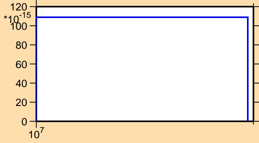
\sigma vs. E for ^{192}\text{Hg}(n,\text{pd})
