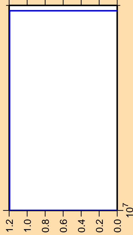
\Delta\sigma/\sigma vs. E for ^{192}\text{Hg}(n,nt)
