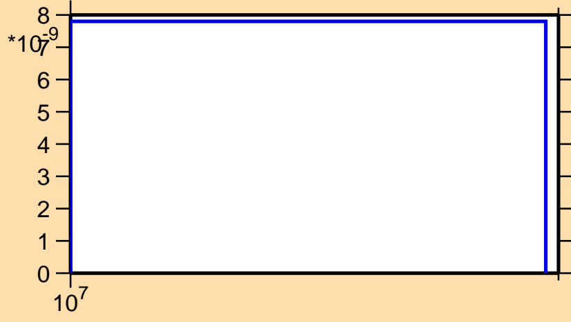
\sigma vs. E for ^{192}\text{Hg}(n,2n\alpha)
