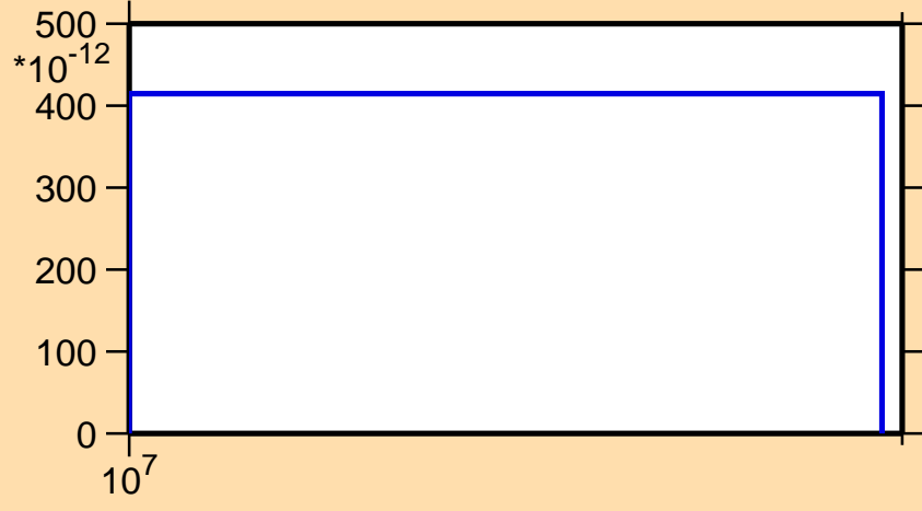
\sigma vs. E for ^{192}\text{Hg}(n,\text{He}3)
