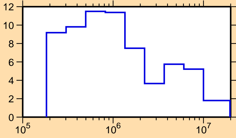
\Delta\sigma/\sigma vs. E for ^{192}\text{Hg}(n,\text{tot.})
