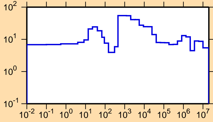
\Delta\sigma/\sigma vs. E for ^{192}\text{Hg}(n,\text{el.})
