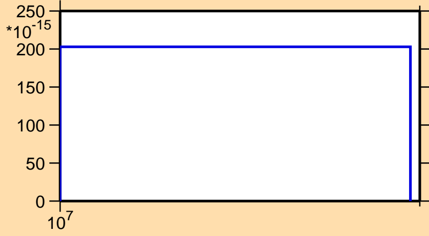
\sigma vs. E for ^{192}\text{Hg} (mt 45)
