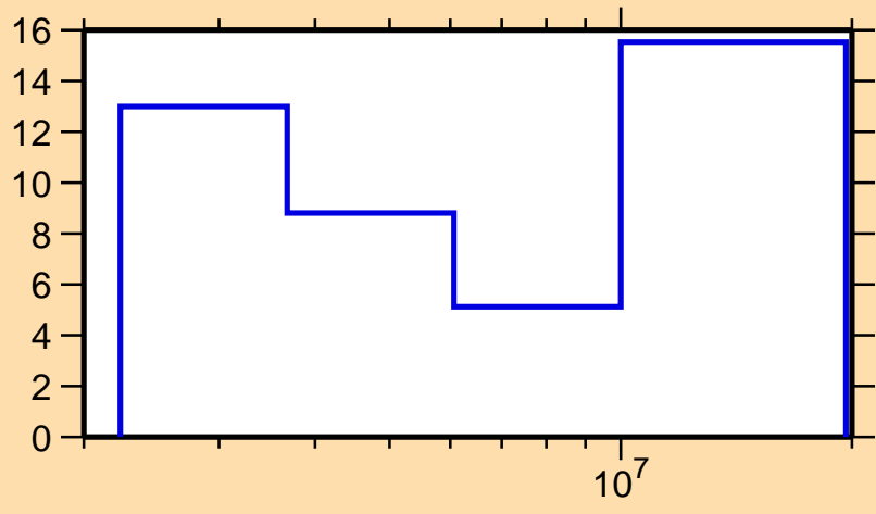
\Delta\sigma/\sigma vs. E for ^{192}\text{Hg}(n,n\text{cont.})
