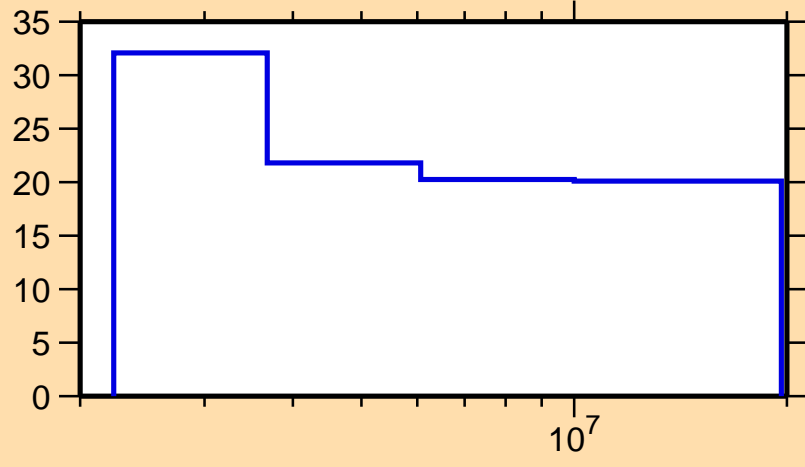
\Delta\sigma/\sigma vs. E for ^{192}\text{Hg}(n,n_1)
