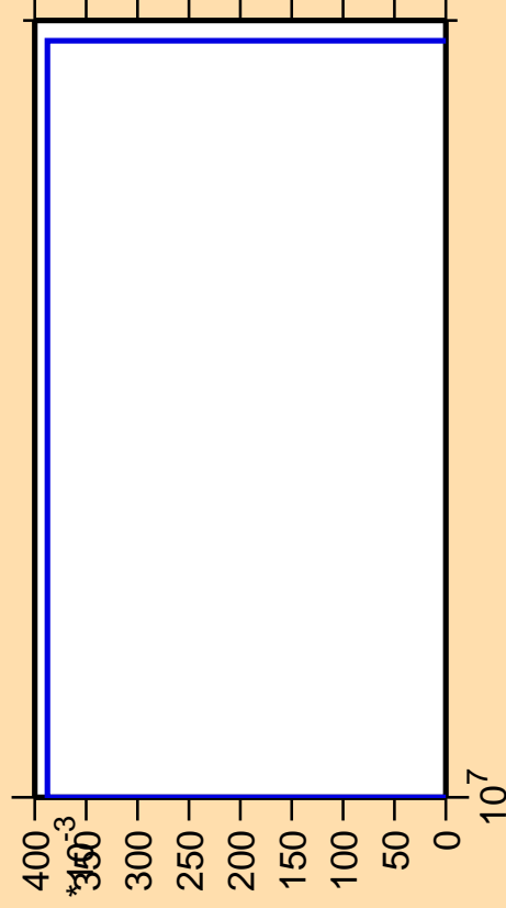
\Delta\sigma/\sigma vs. E for ^{192}\text{Hg}(n,\text{pd})
