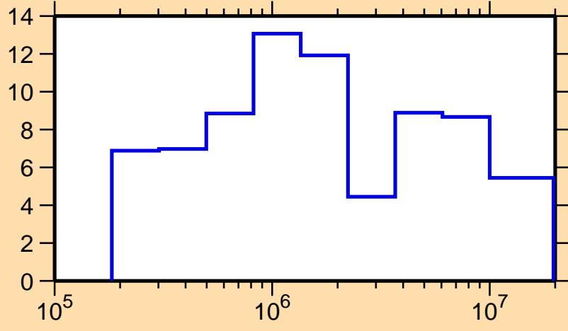
\Delta\sigma/\sigma vs. E for ^{192}\text{Hg}(n,\text{el.})
