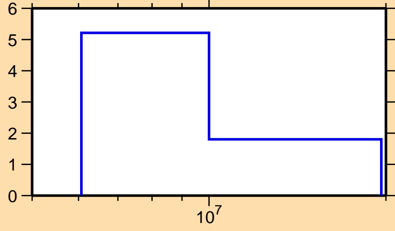
\Delta\sigma/\sigma vs. E for ^{192}\text{Hg}(n,\text{tot.})
