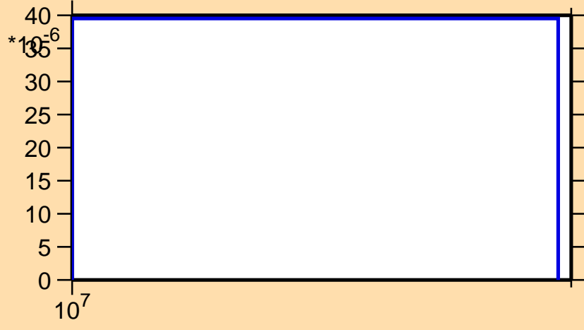
\sigma vs. E for ^{192}\text{Hg}(n,3n)
