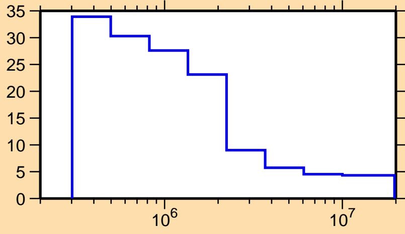
\Delta\sigma/\sigma vs. E for ^{192}\text{Hg}(n,\text{nonel.})
