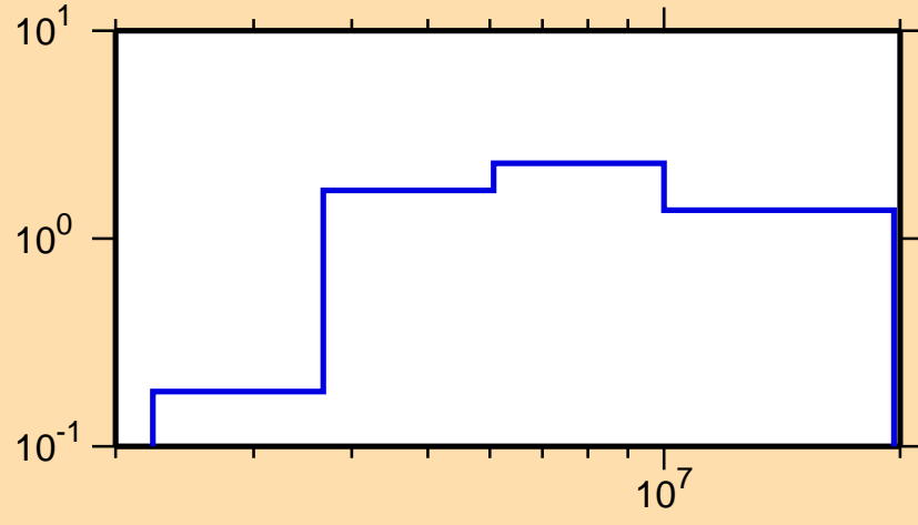
\sigma vs. E for ^{192}\text{Hg}(n,n\text{cont.})
