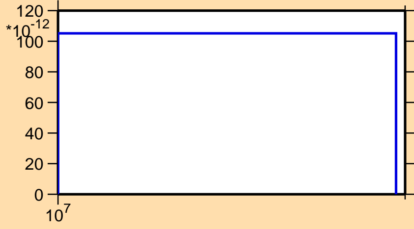
\sigma vs. E for ^{192}\text{Hg}(n,2np)
