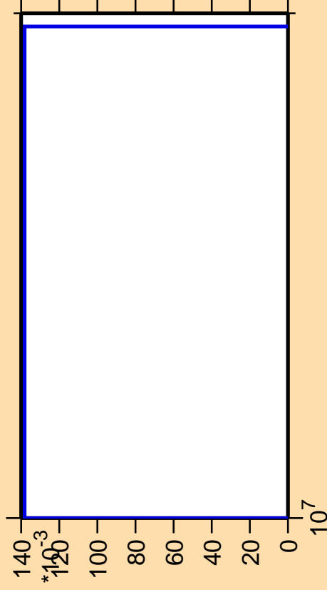
\Delta\sigma/\sigma vs. E for ^{192}\text{Hg}(\text{mt117})
