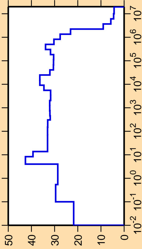
\Delta\sigma/\sigma vs. E for ^{192}\text{Hg}(n,\text{nonel.})
