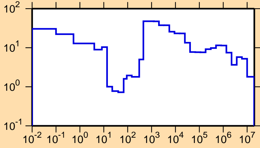
\Delta\sigma/\sigma vs. E for ^{192}\text{Hg}(n,\text{tot.})
