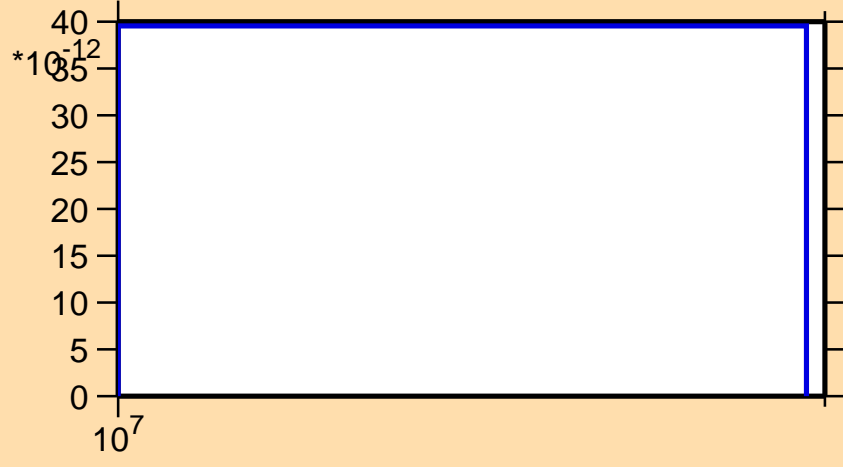
\sigma vs. E for ^{192}\text{Hg}(n,\text{nd})
