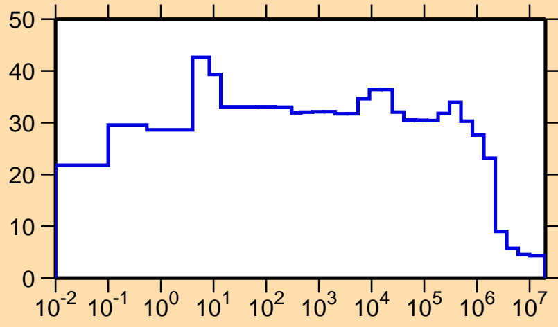
\Delta\sigma/\sigma vs. E for ^{192}\text{Hg}(n,\text{nonel.})
