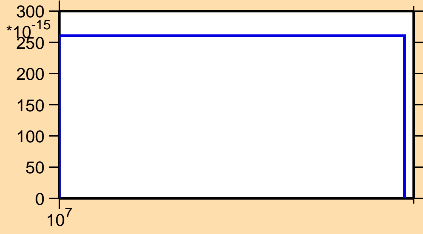
\sigma vs. E for ^{192}\text{Hg}(n,nt)
