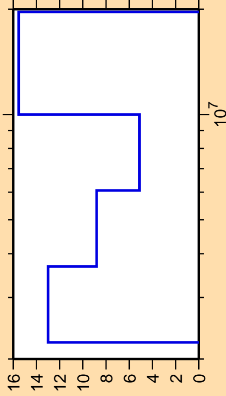
\Delta\sigma/\sigma vs. E for ^{192}\text{Hg}(n,n\text{cont.})
