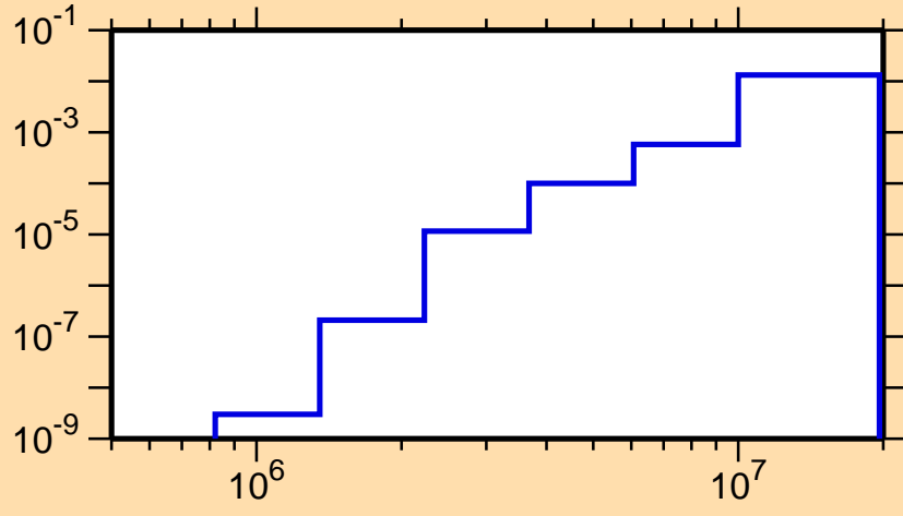
\sigma vs. E for ^{192}\text{Hg}(n,p)
