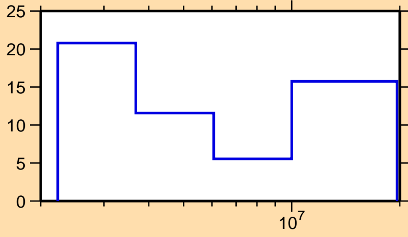
\Delta\sigma/\sigma vs. E for ^{192}\text{Hg}(n,\text{inel.})
