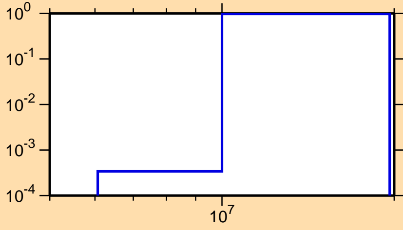
\sigma vs. E for ^{192}\text{Hg}(n,2n)
