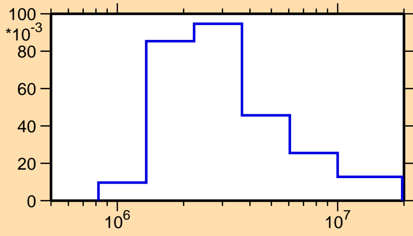
\sigma vs. E for ^{192}\text{Hg}(n,n_2)
