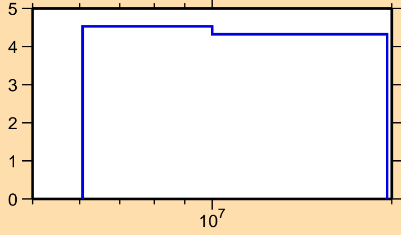
\Delta\sigma/\sigma vs. E for ^{192}\text{Hg}(n,\text{nonel.})
