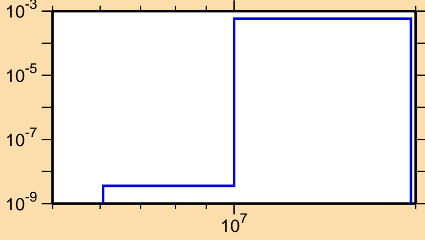
\sigma vs. E for ^{192}\text{Hg}(n,d)
