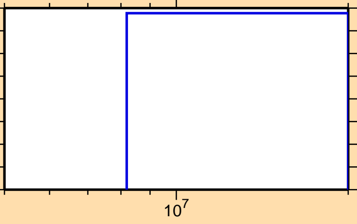
\sigma vs. E for ^{192}\text{Hg}(n,t)
