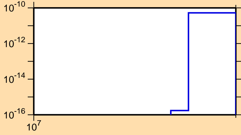
\sigma vs. E for ^{193}\text{Hg}(n,nt)
