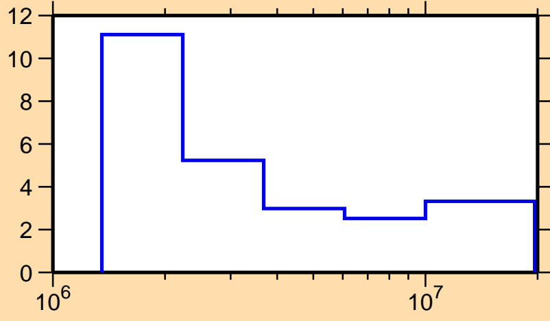
\Delta\sigma/\sigma vs. E for ^{193}\text{Hg}(n,\text{nonel.})
