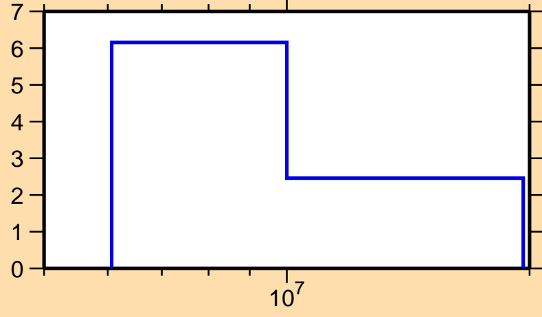
\Delta\sigma/\sigma vs. E for ^{193}\text{Hg}(n,\text{el.})
