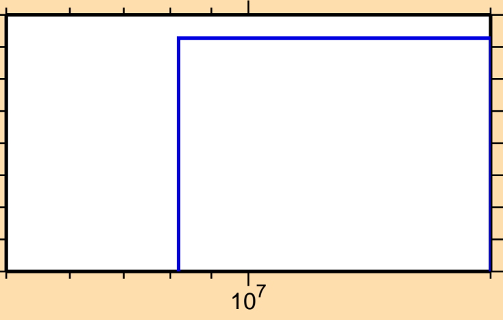
\sigma vs. E for ^{193}\text{Hg}(n,\text{nd})
