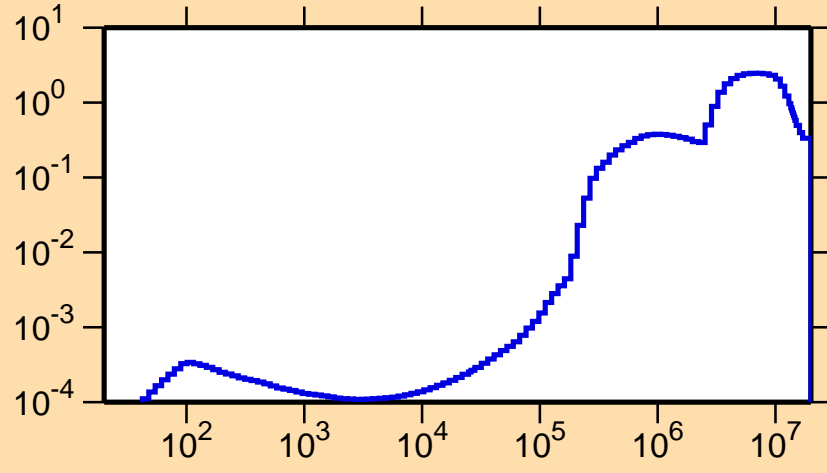
\sigma vs. E for ^{193}\text{Hg}(n,\text{inel.})
