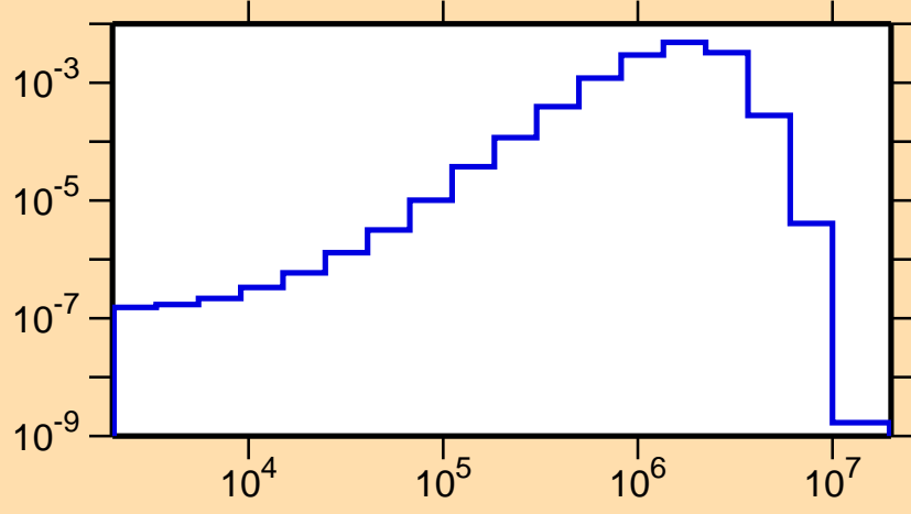
\sigma vs. E for ^{193}\text{Hg}(n,n_1)
