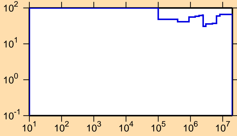
\Delta\sigma/\sigma vs. E for ^{193}\text{Hg}(n,n_1)
