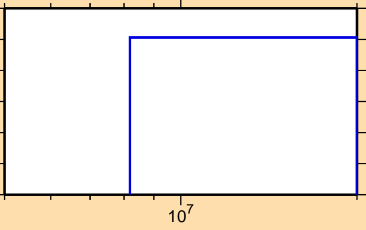
\sigma vs. E for ^{193}\text{Hg}(n,3n)
