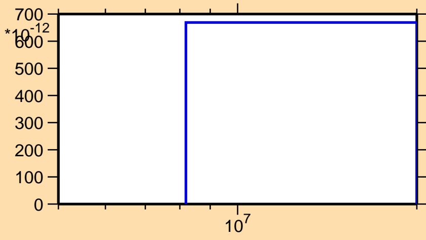
\sigma vs. E for ^{193}\text{Hg}(n,p\alpha)
