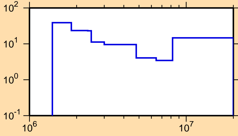
\Delta\sigma/\sigma vs. E for ^{193}\text{Hg}(n,n\text{cont.})
