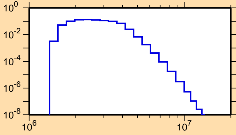
\sigma vs. E for ^{194}\text{Hg}(n,n_4)
