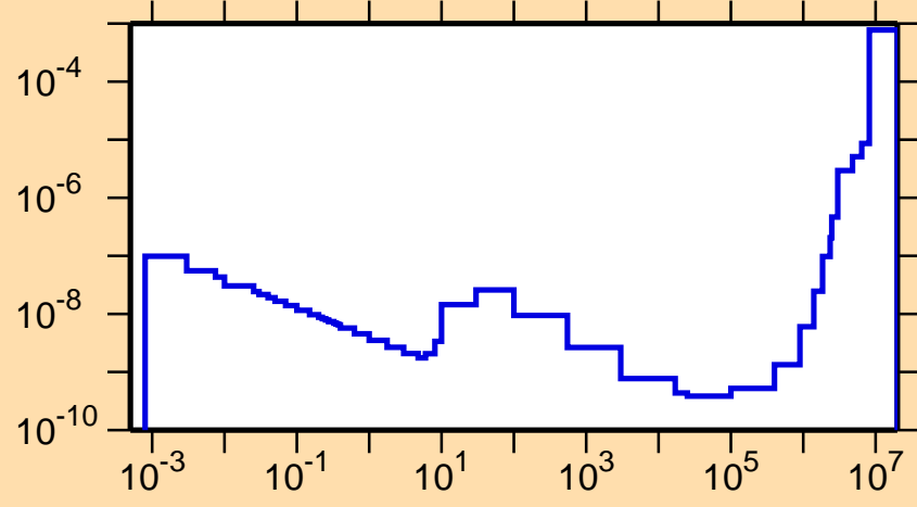
\sigma vs. E for ^{194}\text{Hg}(n,\alpha)
