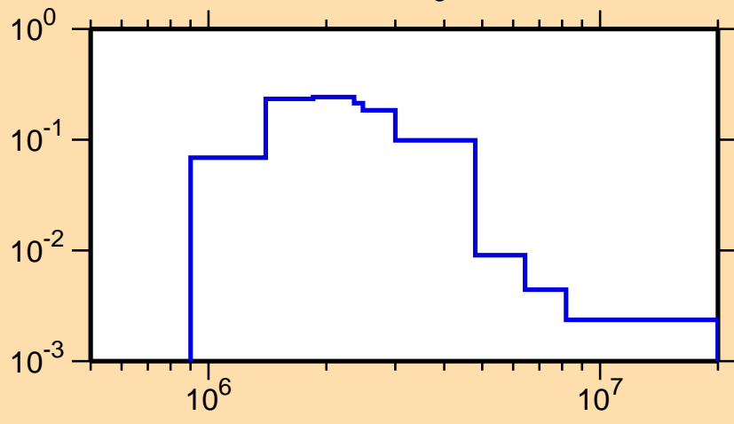
\sigma vs. E for ^{194}\text{Hg}(n,n_3)
