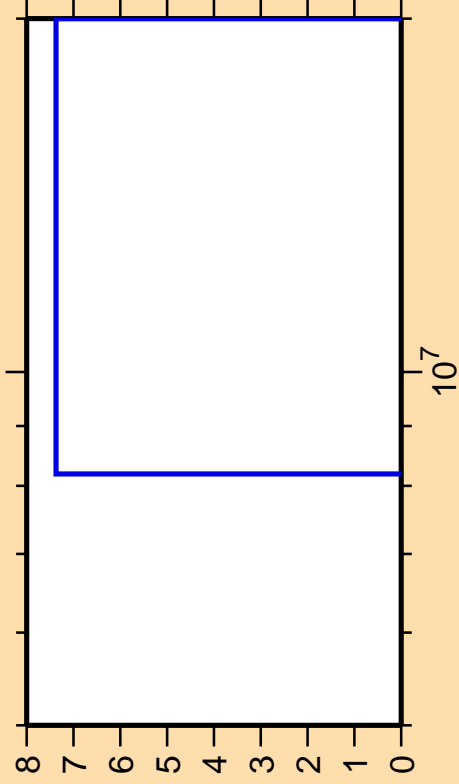
\Delta\sigma/\sigma vs. E for ^{194}\text{Hg}(n,2n)
