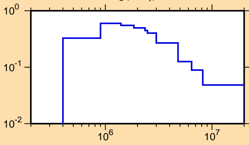
\sigma vs. E for ^{194}\text{Hg}(n,n_1)
