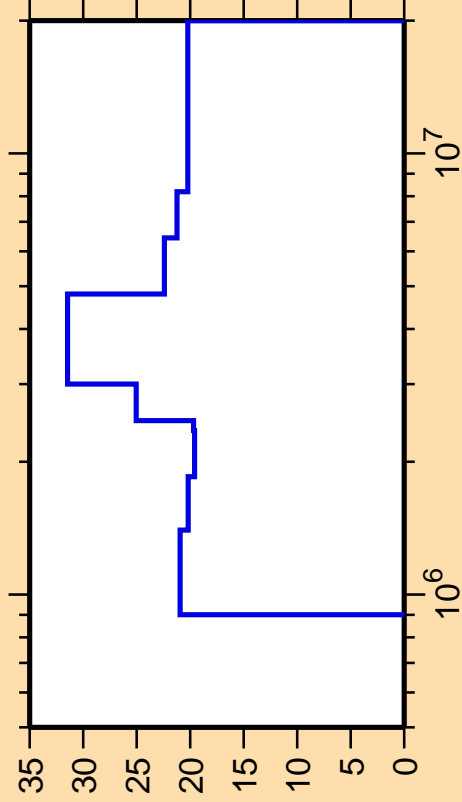
\Delta\sigma/\sigma vs. E for ^{194}\text{Hg}(n,n_3)
