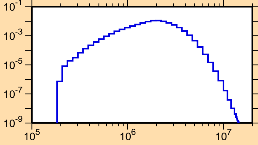
\sigma vs. E for ^{195}\text{Hg}(n,n_3)
