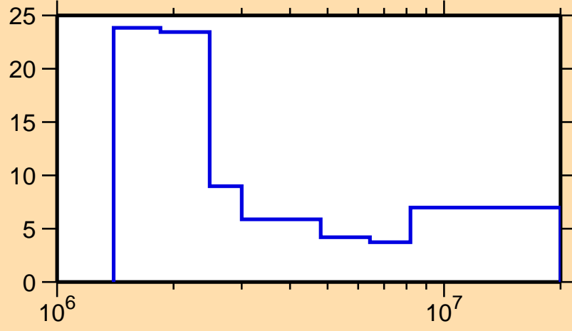
\Delta\sigma/\sigma vs. E for ^{195}\text{Hg}(n,n\text{cont.})
