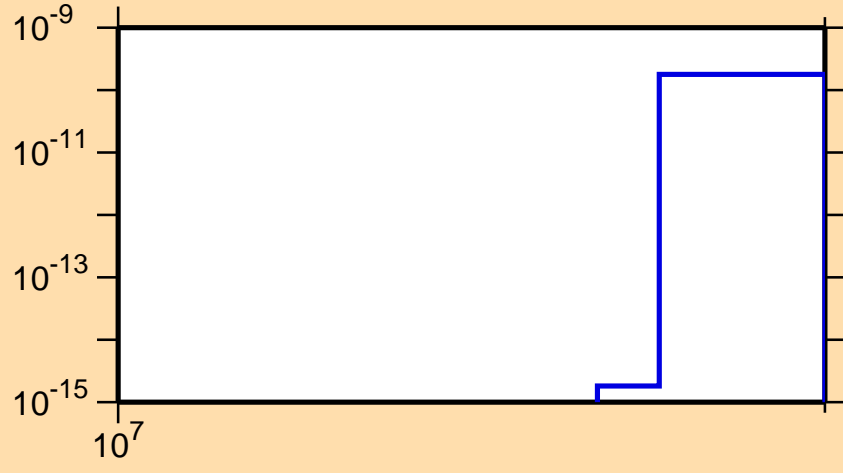
\sigma vs. E for ^{195}\text{Hg}(n,nt)
