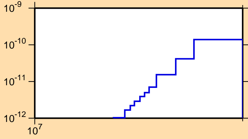
\sigma vs. E for ^{195}\text{Hg}(n,p\alpha)
