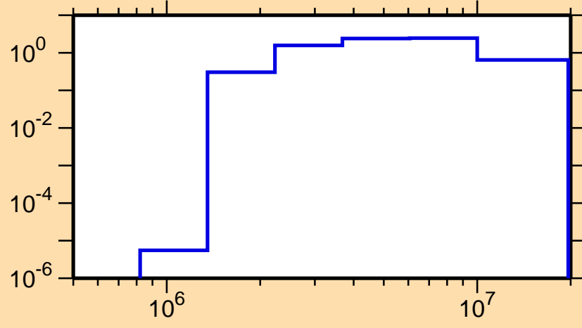
\sigma vs. E for ^{195}\text{Hg}(n,n\text{cont.})
