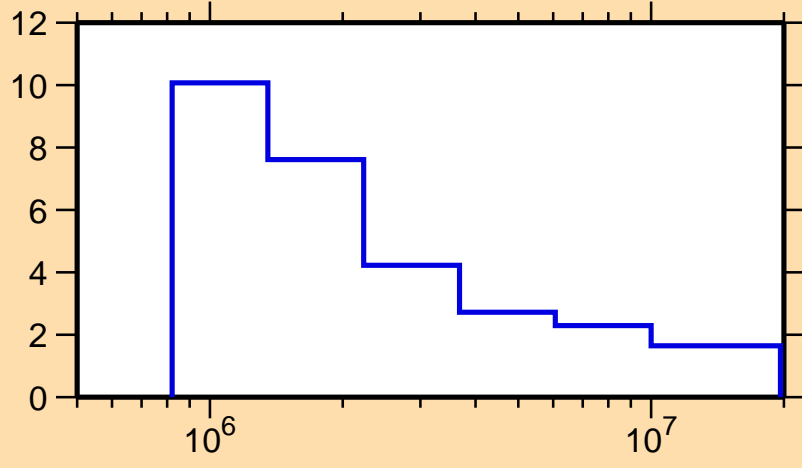
\Delta\sigma/\sigma vs. E for ^{195}\text{Hg}(n,\text{nonel.})
