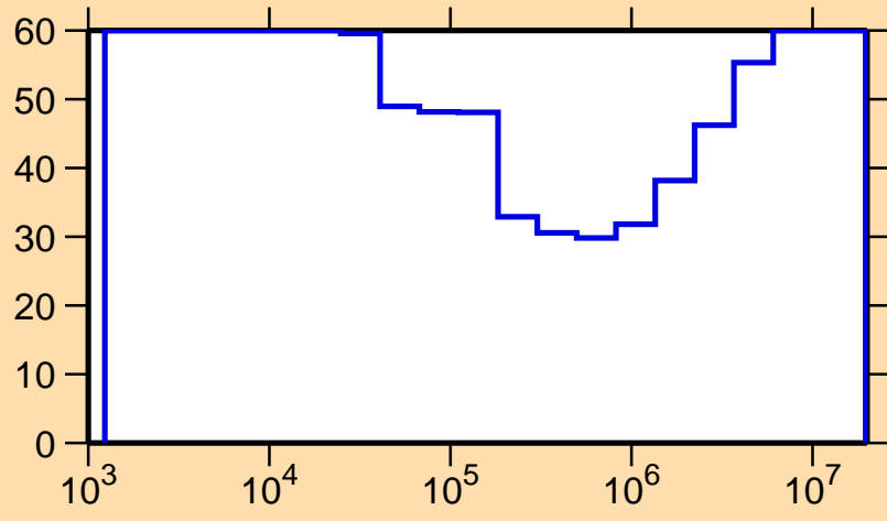
\Delta\sigma/\sigma vs. E for ^{195}\text{Hg}(n,n_1)
