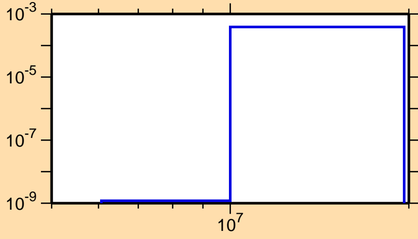
\sigma vs. E for ^{195}\text{Hg}(n,np)
