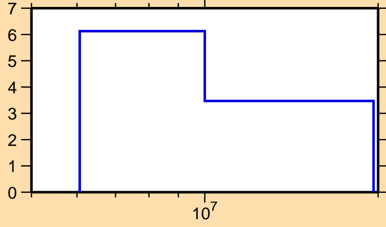
\Delta\sigma/\sigma vs. E for ^{195}\text{Hg}(n,\text{el.})
