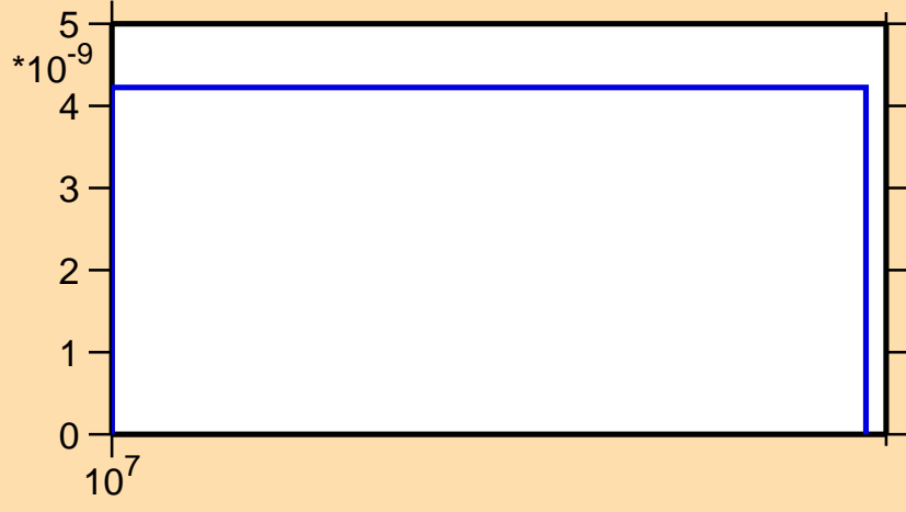
\sigma vs. E for ^{195}\text{Hg}(n,\text{nd})
