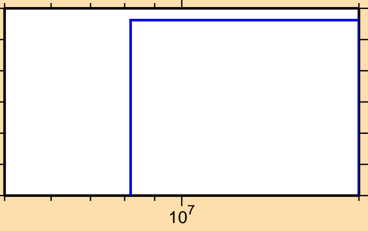
\sigma vs. E for ^{195}\text{Hg}(n,2np)
