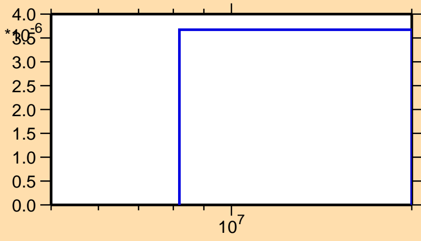
\sigma vs. E for ^{196}\text{Hg}(n,t)
