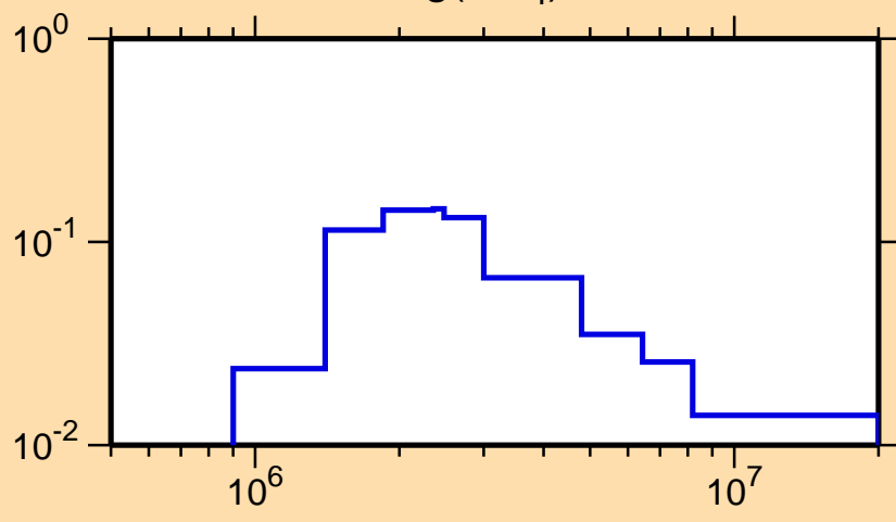
\sigma vs. E for ^{196}\text{Hg}(n,n_4)
