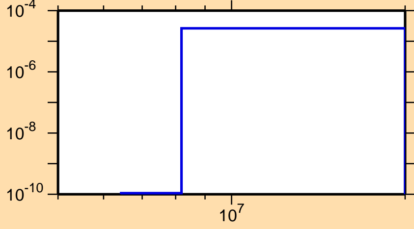
\sigma vs. E for ^{196}\text{Hg}(n,n\alpha)
