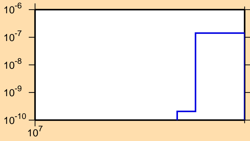
\sigma vs. E for ^{197}\text{Hg}(n,2np)
