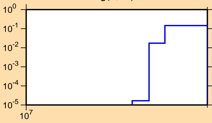
\sigma vs. E for ^{197}\text{Hg}(n,3n)
