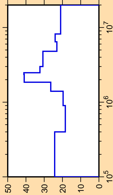
\Delta\sigma/\sigma vs. E for ^{197}\text{Hg}(n,n_2)
