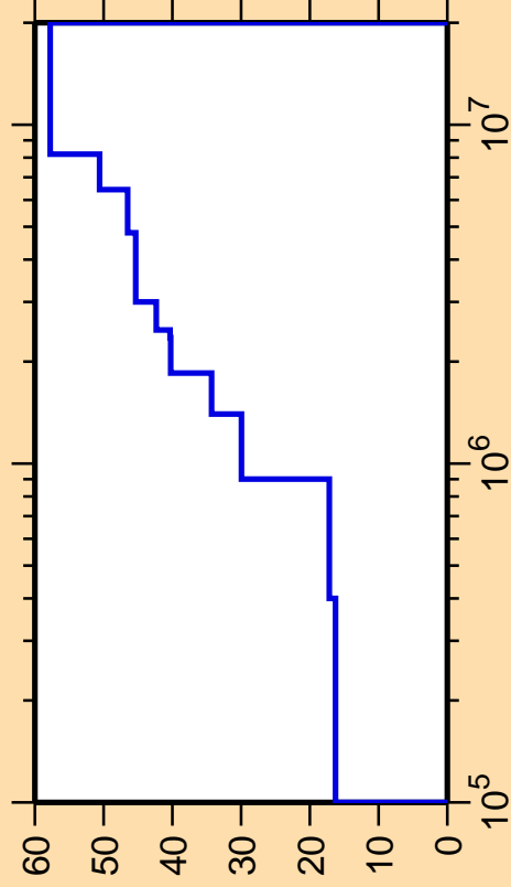
\Delta\sigma/\sigma vs. E for ^{197}\text{Hg}(n,n_4)
