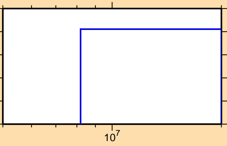
\sigma vs. E for ^{197}\text{Hg}(n,\text{He}3)
