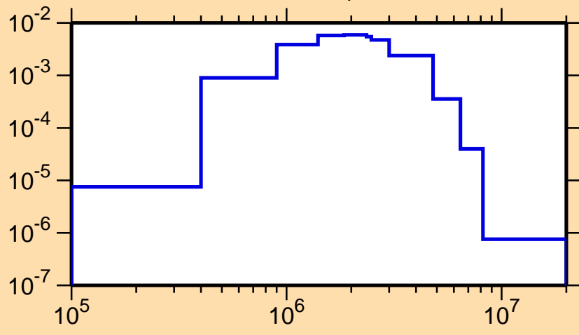
\sigma vs. E for ^{197}\text{Hg}(n,n_4)
