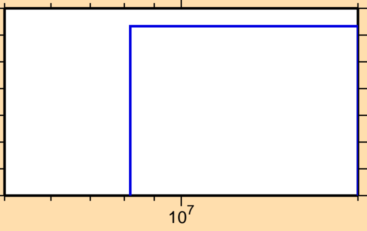
\sigma vs. E for ^{197}\text{Hg}(n,t)
