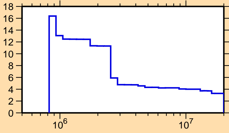
\Delta\sigma/\sigma vs. E for ^{197}\text{Hg}(n,n\text{onel.})
