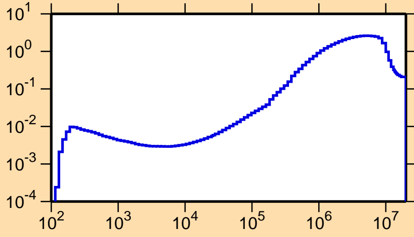
\sigma vs. E for ^{197}\text{Hg}(n,\text{inel.})
