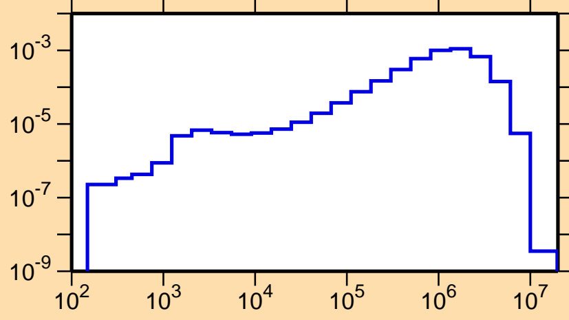
\sigma vs. E for ^{197}\text{Hg}(n,n_1)
