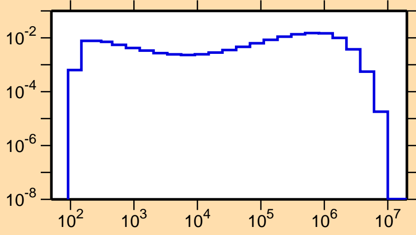
\sigma vs. E for ^{197}\text{Hg}(n,n_2)
