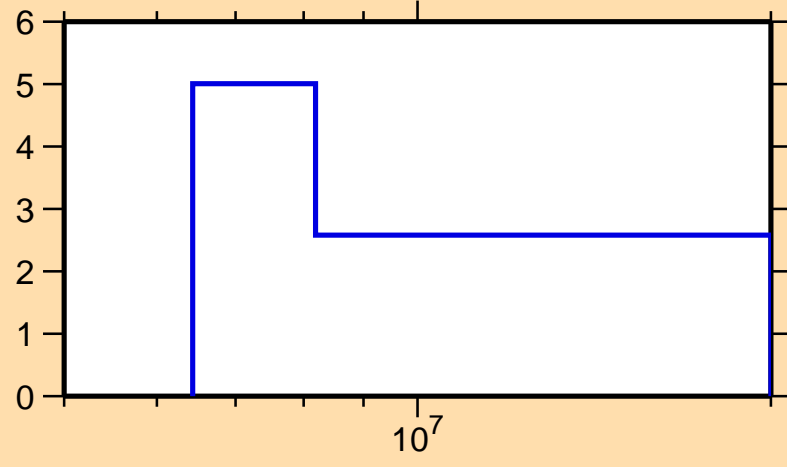
\Delta\sigma/\sigma vs. E for ^{197}\text{Hg}(n,\text{el.})
