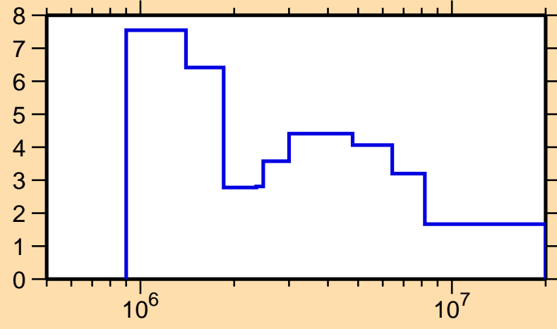
\Delta\sigma/\sigma vs. E for ^{197}\text{Hg}(n,\text{tot.})
