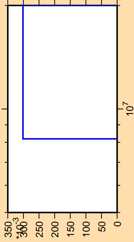
\Delta\sigma/\sigma vs. E for ^{197}\text{Hg}(n,p\alpha)
