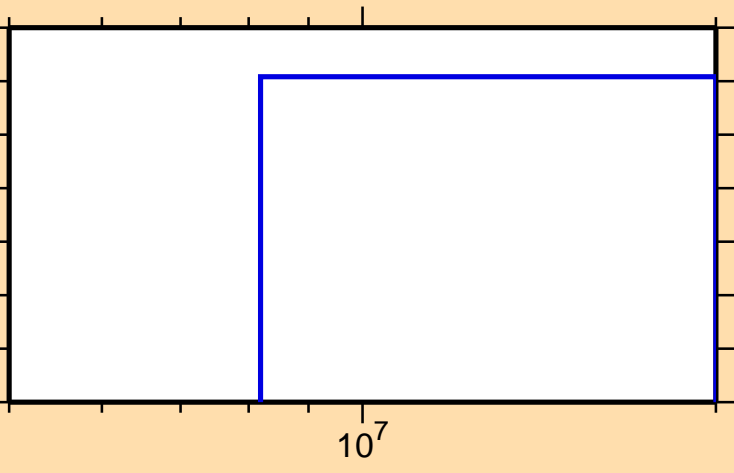
\sigma vs. E for ^{197}\text{Hg}(n,p\alpha)
