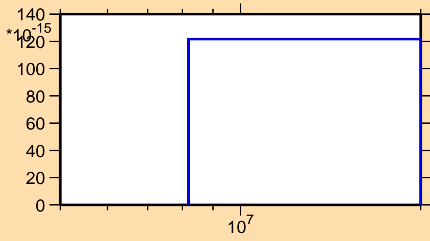
\sigma vs. E for ^{197}\text{Hg}(n,p\alpha)
